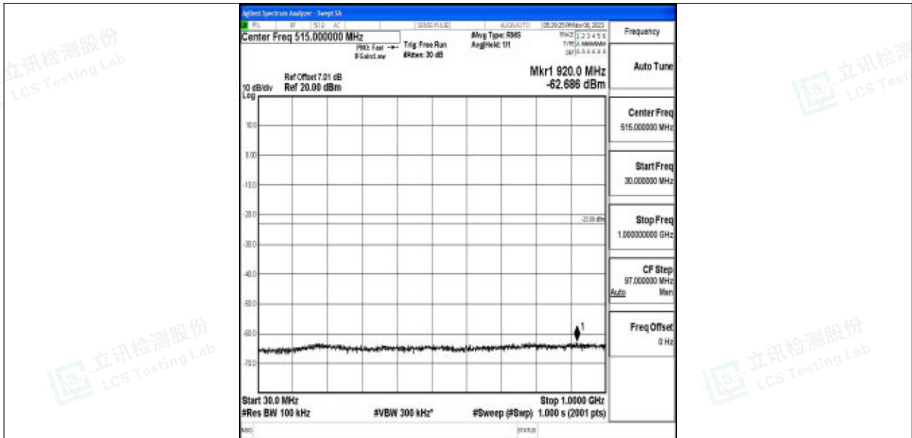
Band2_20MHz_QPSK_19100_1RB#0_30~1000_30~1000
