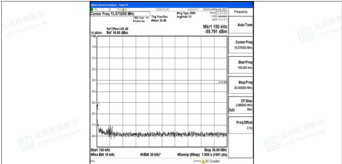
Band2_5MHz_QPSK_19175_1RB#0_0.15~30_0.15~30
