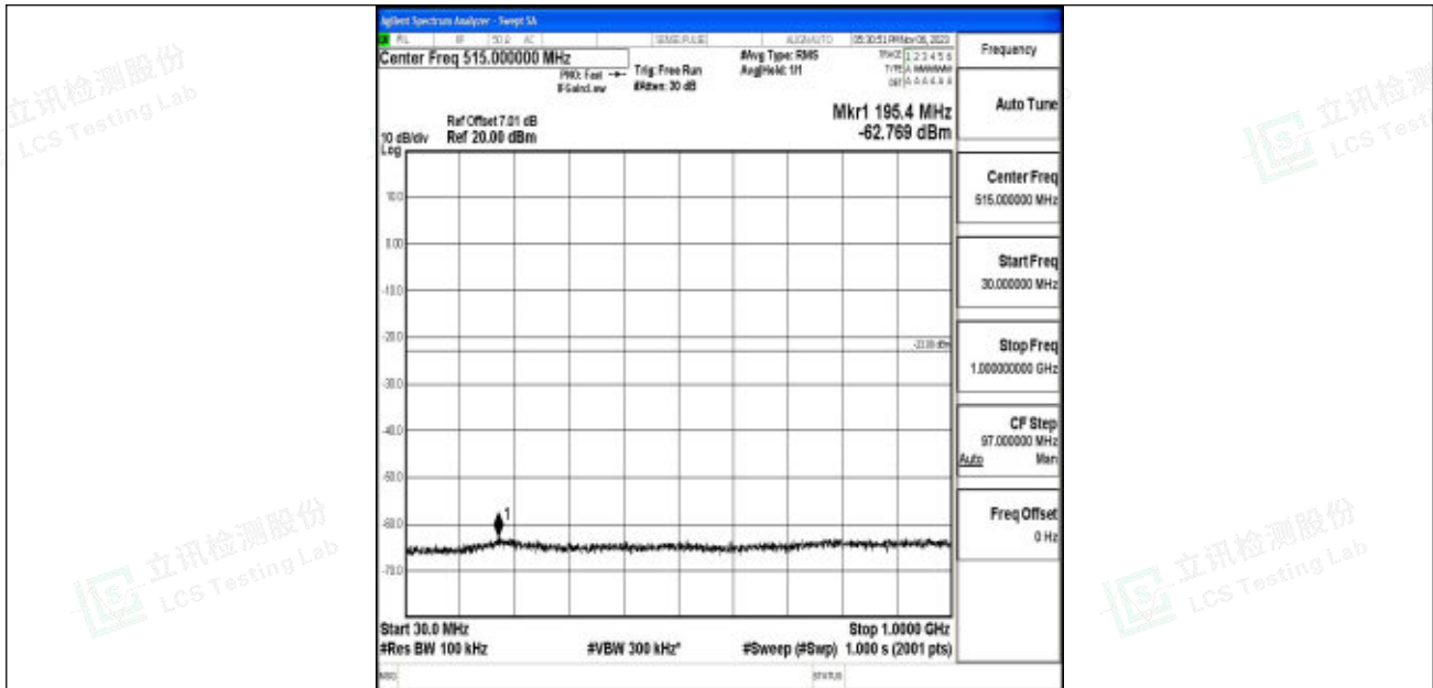
Band2_20MHz_64QAM_19100_1RB#0_30~1000_30~1000
