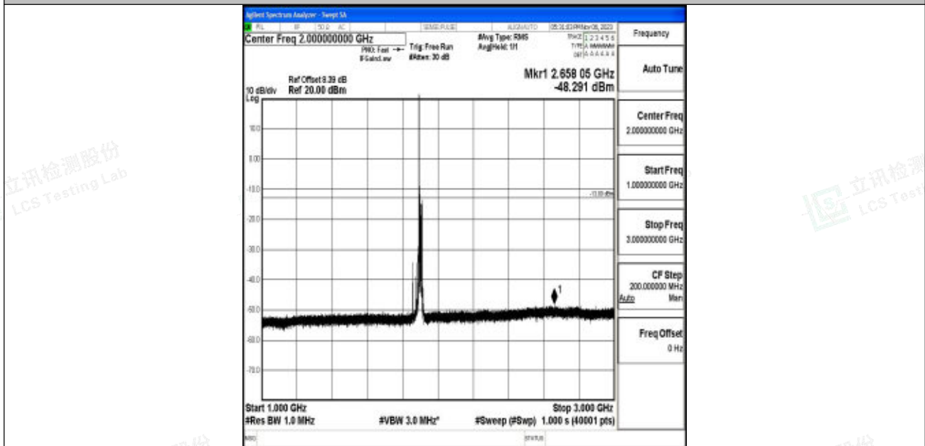
Band2_20MHz_64QAM_19100_1RB#0_1000~3000_1000~3000
