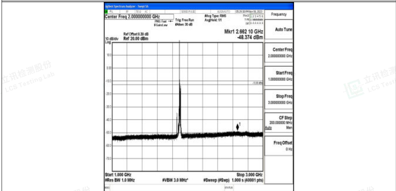
Band2_20MHz_QPSK_19100_1RB#0_1000~3000_1000~3000
