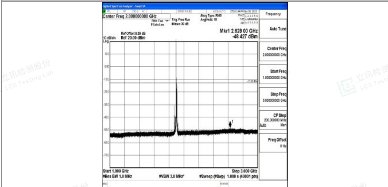
Band2_15MHz_16QAM_19125_1RB#0_1000~3000_1000~3000
