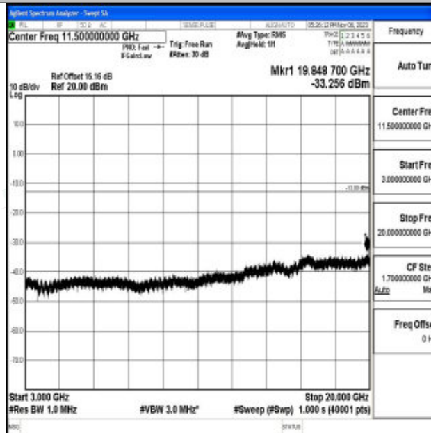
Band2_20MHz_16QAM_18700_1RB#0_3000~20000_3000~20000
