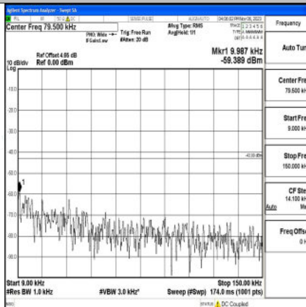
Band2_5MHz_64QAM_19175_1RB#0_0.009~0.15_0.009~0.15
