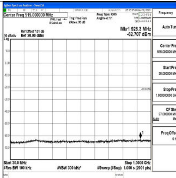
Band2_20MHz_QPSK_18700_1RB#0_30~1000_30~1000
