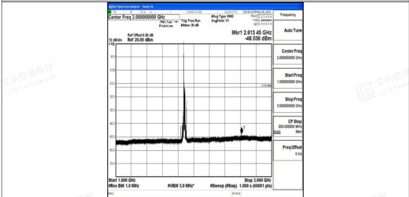
Band2_20MHz_16QAM_18900_1RB#0_1000~3000_1000~3000
