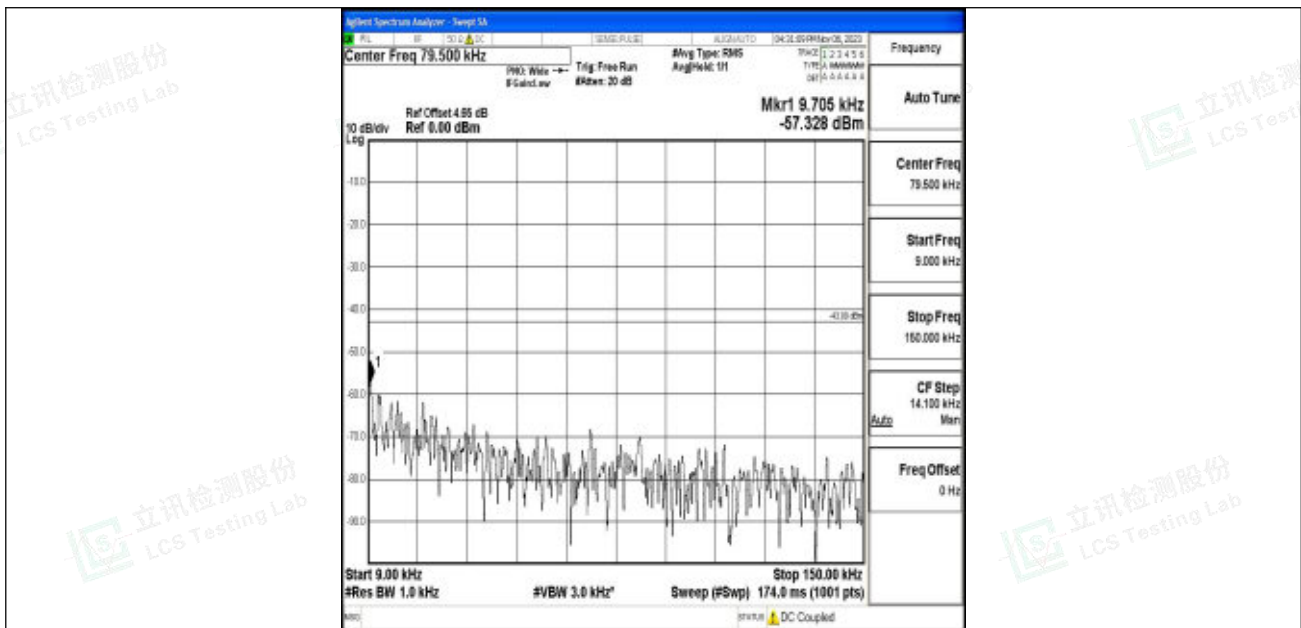
Band2_10MHz_QPSK_19150_1RB#0_0.009~0.15_0.009~0.15
