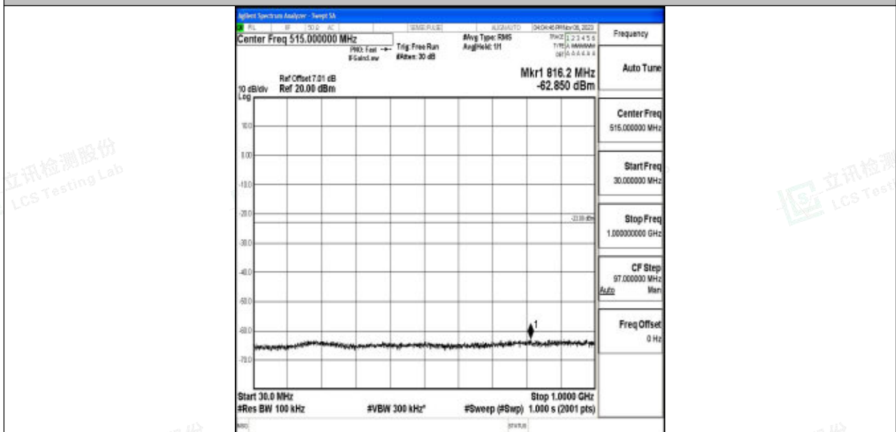
Band2_5MHz_QPSK_19175_1RB#0_30~1000_30~1000
