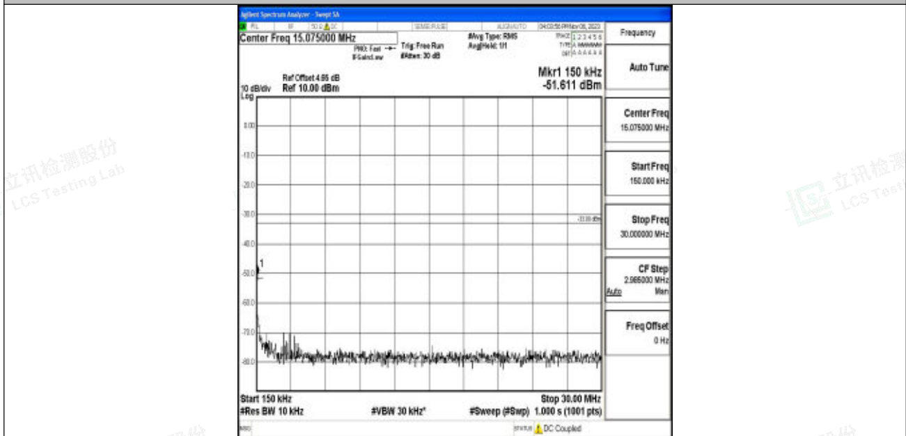
Band2_5MHz_64QAM_18900_1RB#0_0.15~30_0.15~30
