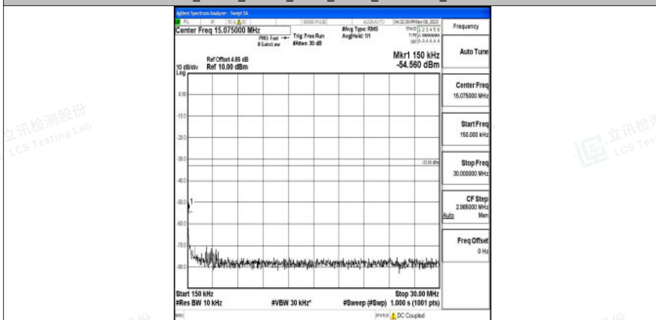
Band2_10MHz_64QAM_19150_1RB#0_0.15~30_0.15~30
