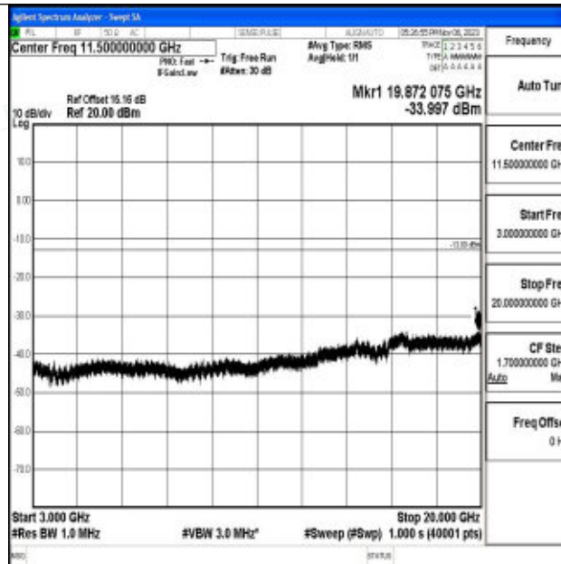
Band2_20MHz_64QAM_18700_1RB#0_3000~20000_3000~20000
