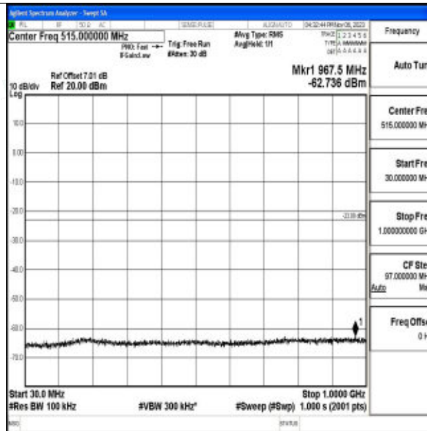
Band2_10MHz_64QAM_19150_1RB#0_30~1000_30~1000
