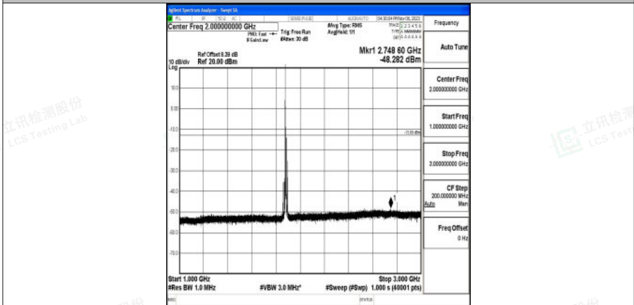
Band2_10MHz_16QAM_18900_1RB#0_1000~3000_1000~3000
