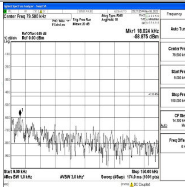
Band2_20MHz_QPSK_18900_1RB#0_0.009~0.15_0.009~0.15
