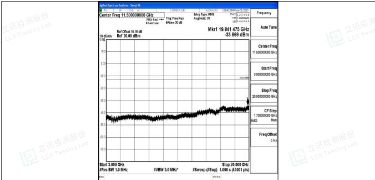
Band2_15MHz_64QAM_18900_1RB#0_3000~20000_3000~20000
