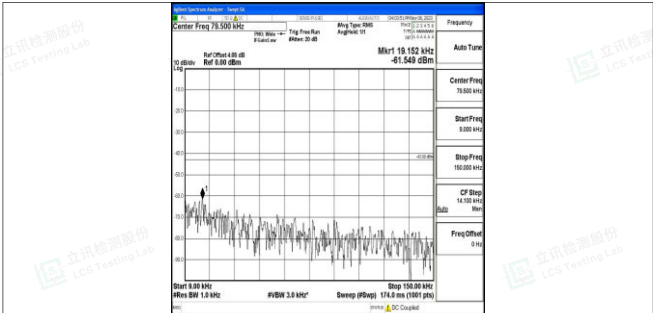
Band2_5MHz_64QAM_18900_1RB#0_0.009~0.15_0.009~0.15
