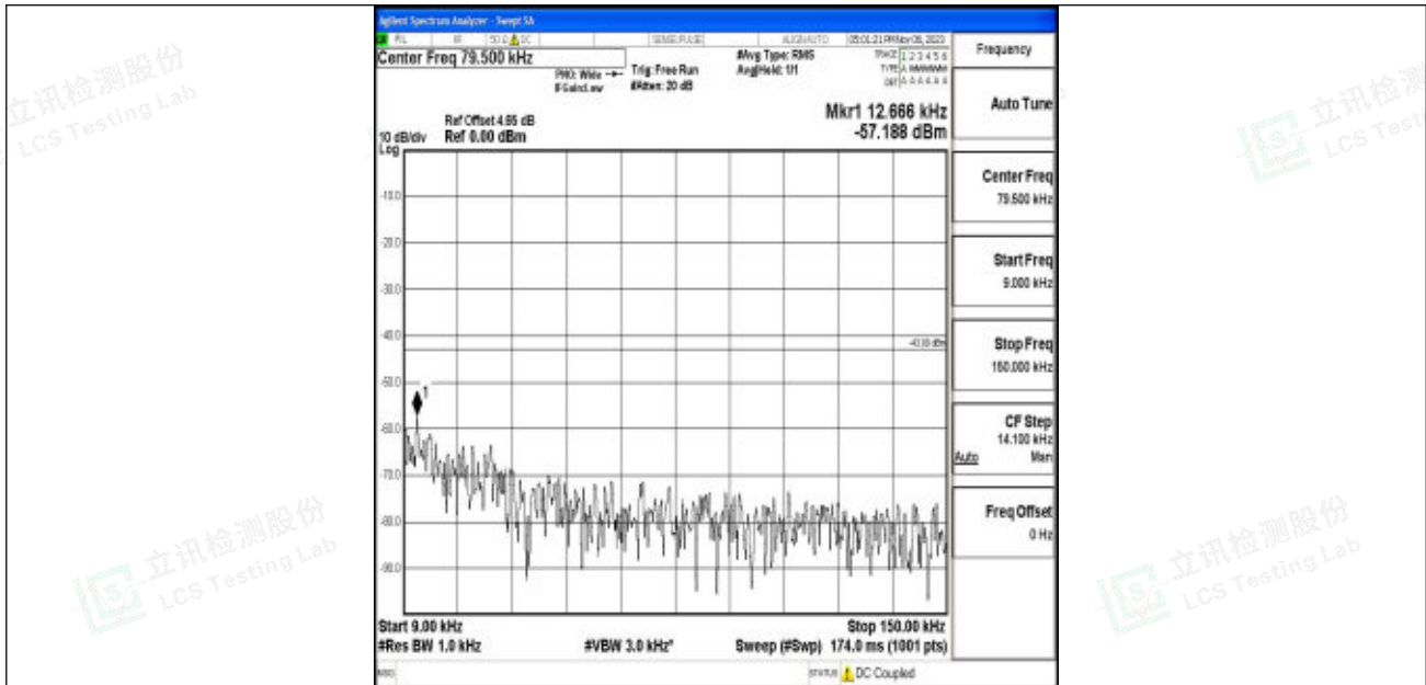
Band2_15MHz_16QAM_19125_1RB#0_0.009~0.15_0.009~0.15
