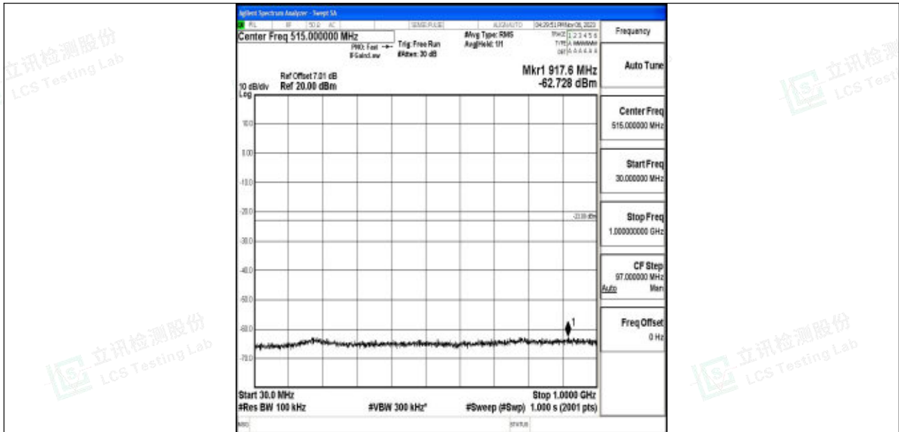
Band2_10MHz_16QAM_18900_1RB#0_30~1000_30~1000
