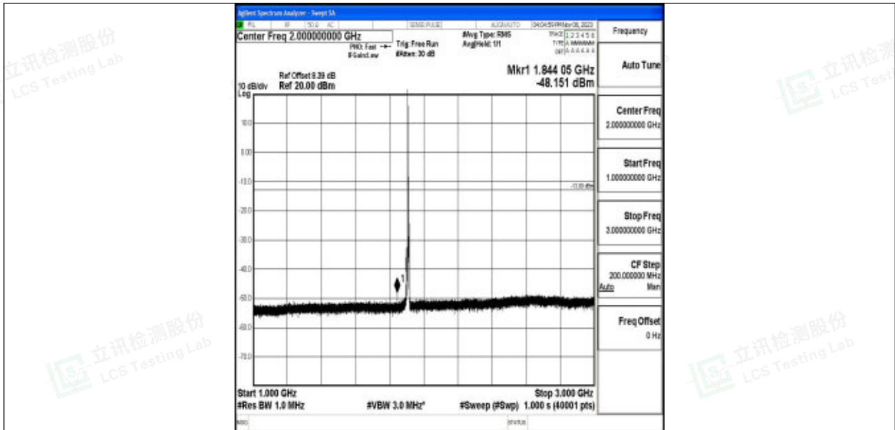
Band2_5MHz_QPSK_19175_1RB#0_1000~3000_1000~3000
