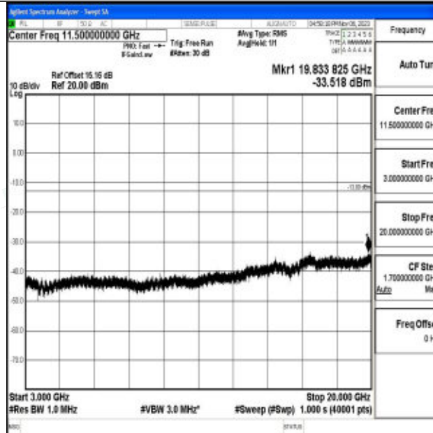
Band2_15MHz_64QAM_18675_1RB#0_3000~20000_3000~20000
