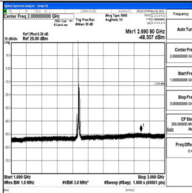
Band2_15MHz_64QAM_18900_1RB#0_1000~3000_1000~3000
