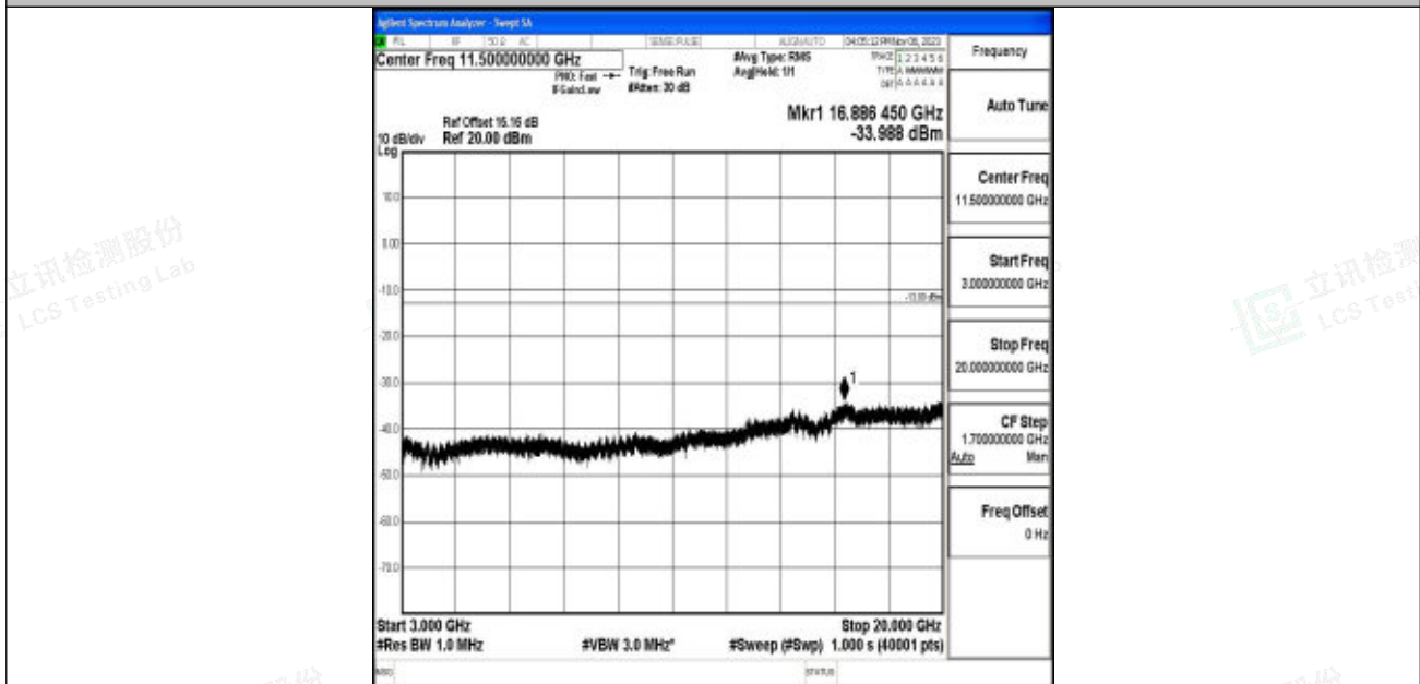
Band2_5MHz_QPSK_19175_1RB#0_3000~20000_3000~20000
