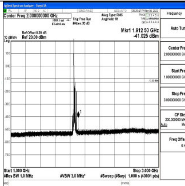
Band2_20MHz_QPSK_18700_1RB#0_1000~3000_1000~3000
