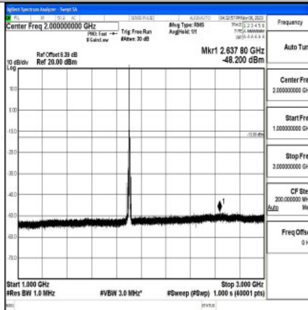
Band2_10MHz_64QAM_19150_1RB#0_1000~3000_1000~3000
