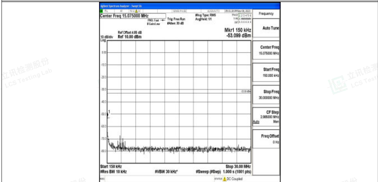
Band2_15MHz_16QAM_19125_1RB#0_0.15~30_0.15~30
