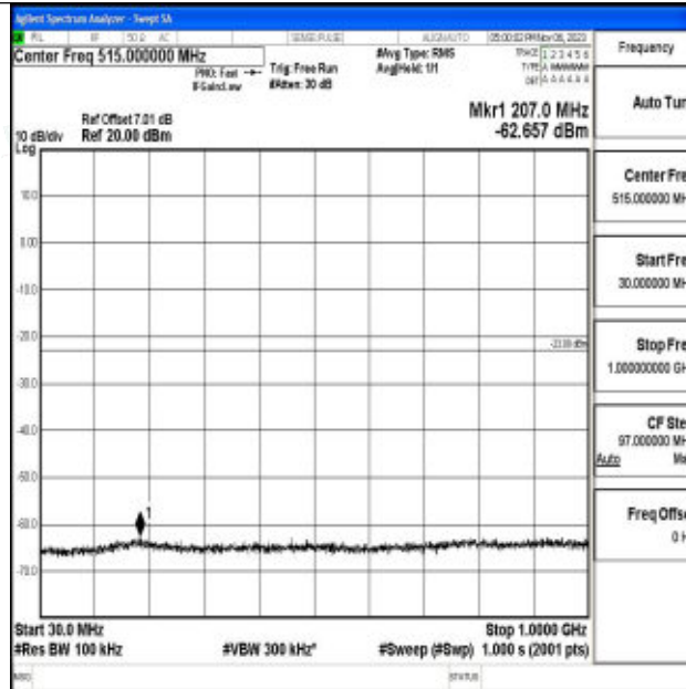
Band2_15MHz_64QAM_18900_1RB#0_30~1000_30~1000
