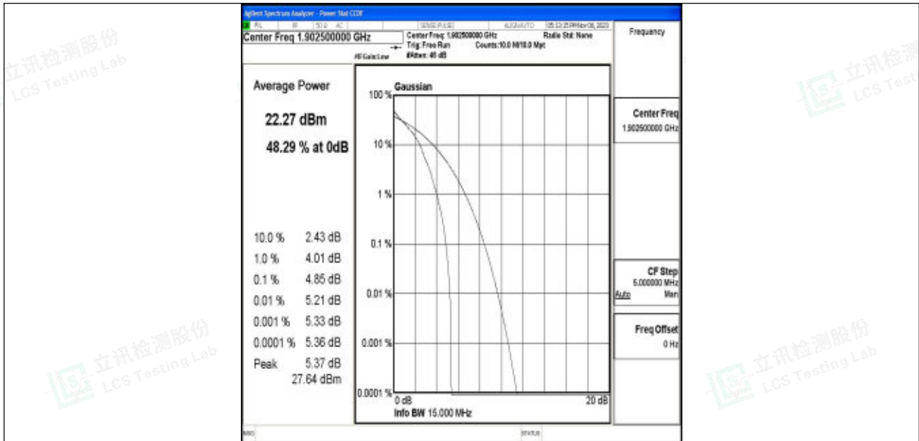
Band2-15MHz-64QAM-19125-1RB#0-PASS
