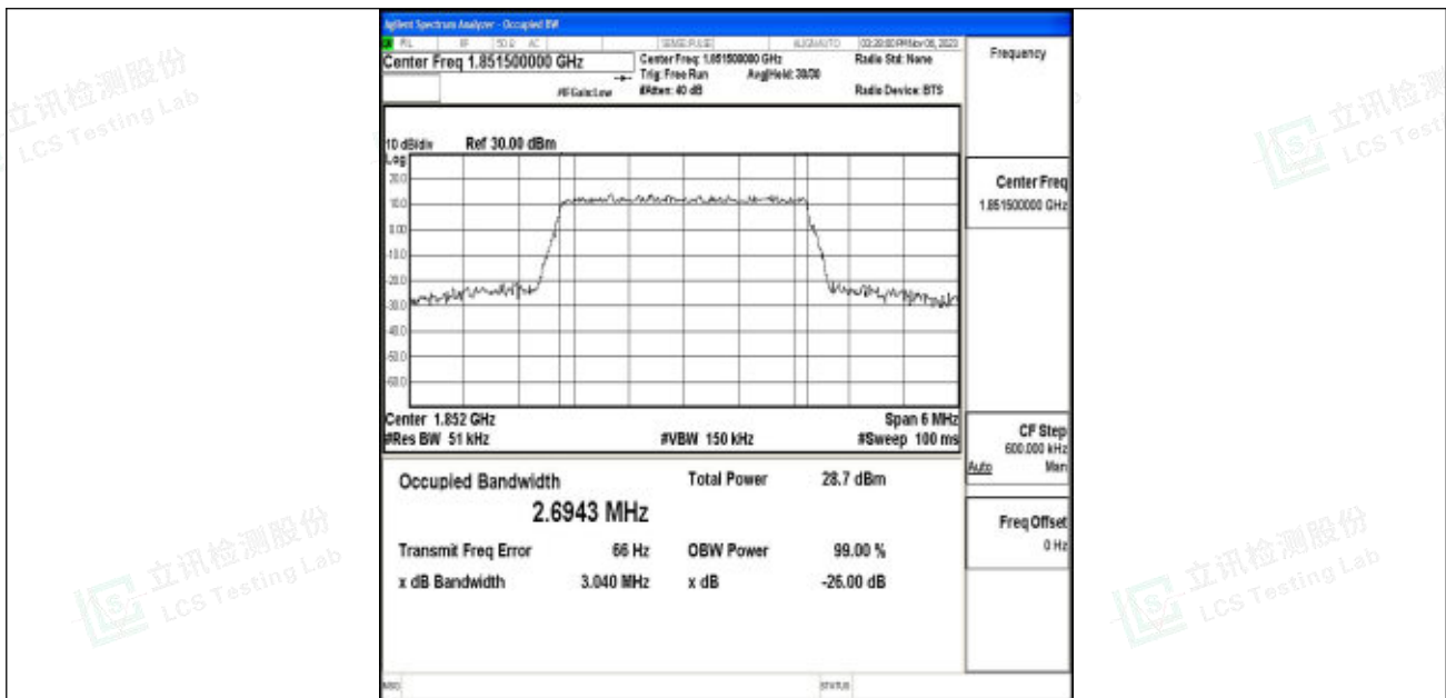
Band2-3MHz-16QAM-18615-15RB#0-PASS
