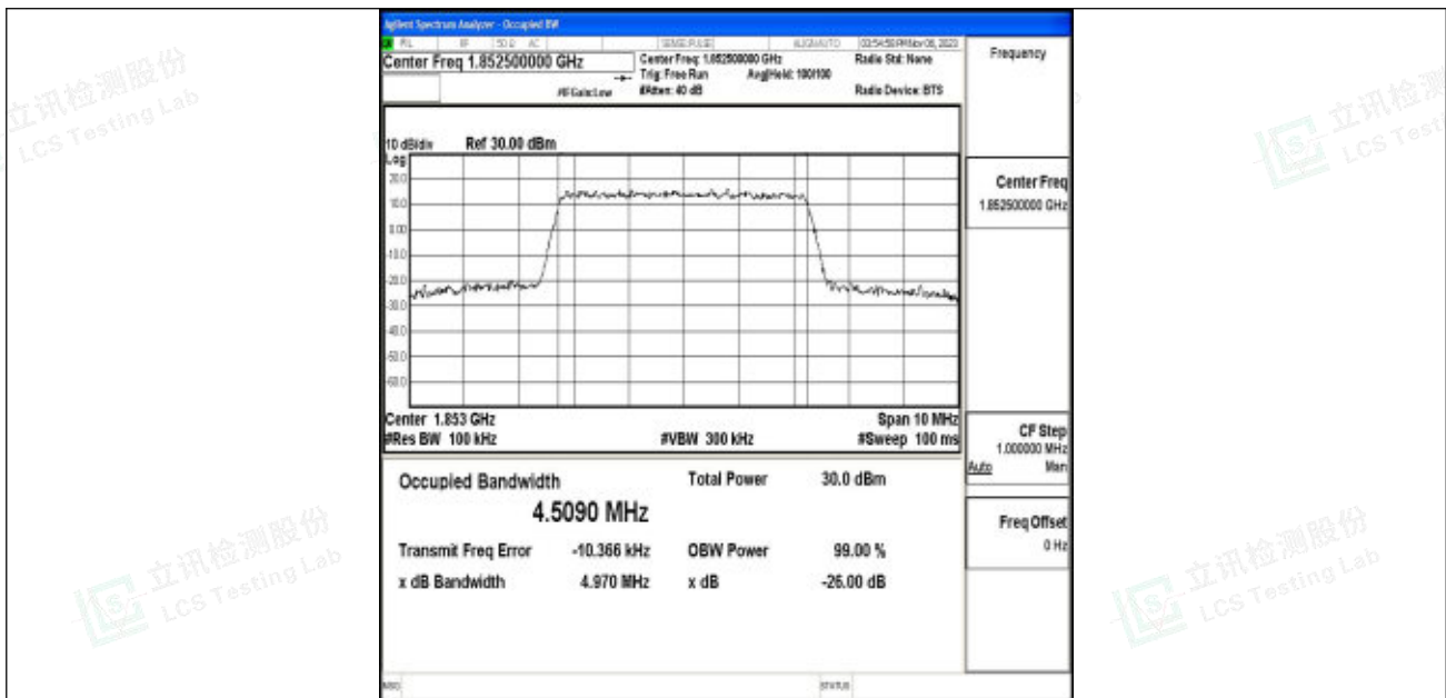
Band2-5MHz-64QAM-18625-25RB#0-PASS
