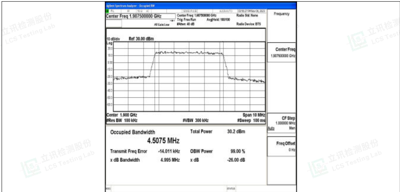
Band2-5MHz-QPSK-19175-25RB#0-PASS
