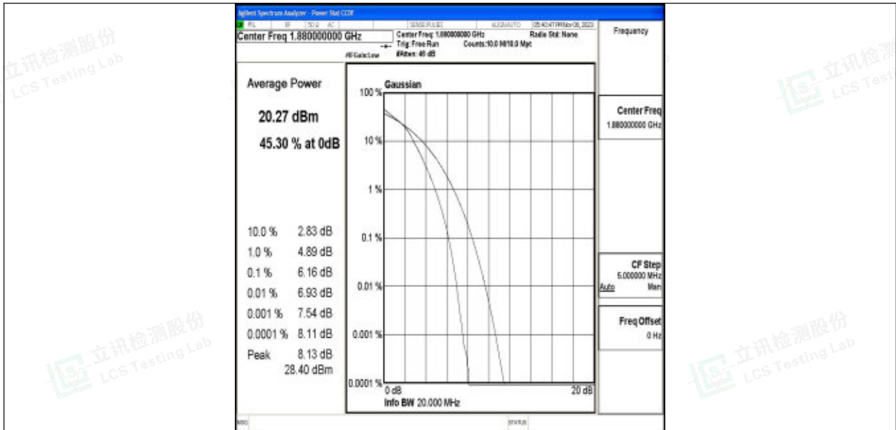
Band2-20MHz-16QAM-18900-100RB#0-PASS
