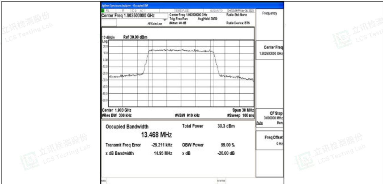
Band2-15MHz-64QAM-19125-75RB#0-PASS
