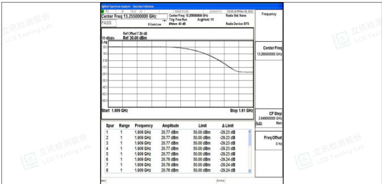
Band2_1.4MHz_16QAM_19193_1RB#0
