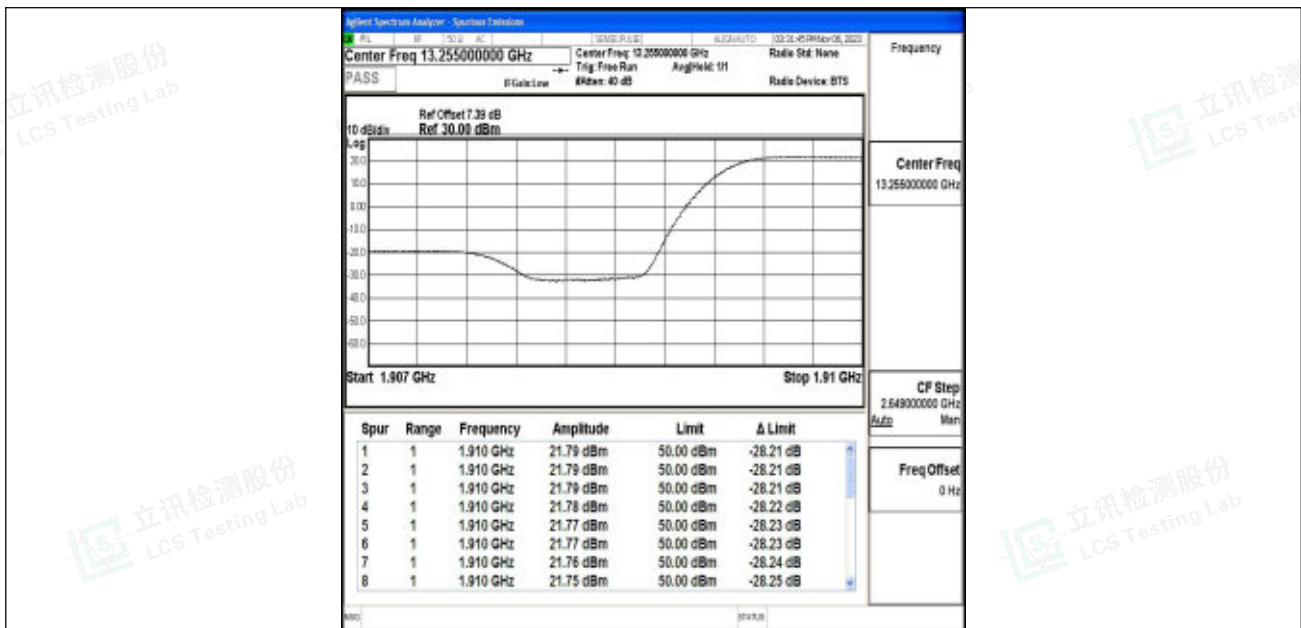
Band2_3MHz_64QAM_19185_1RB#14
