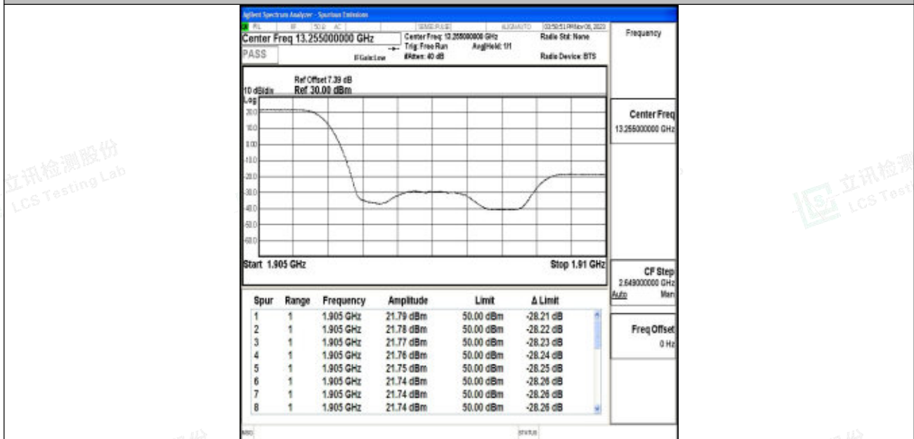
Band2_5MHz_QPSK_19175_1RB#0
