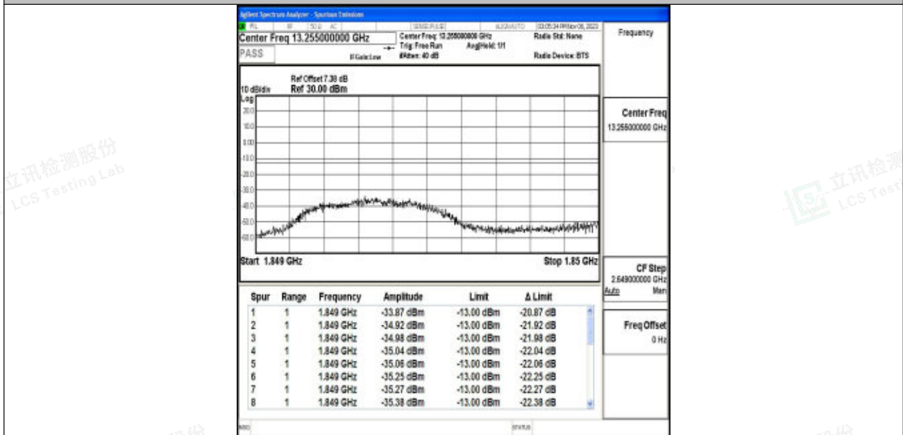
Band2_1.4MHz_64QAM_18607_1RB#5
