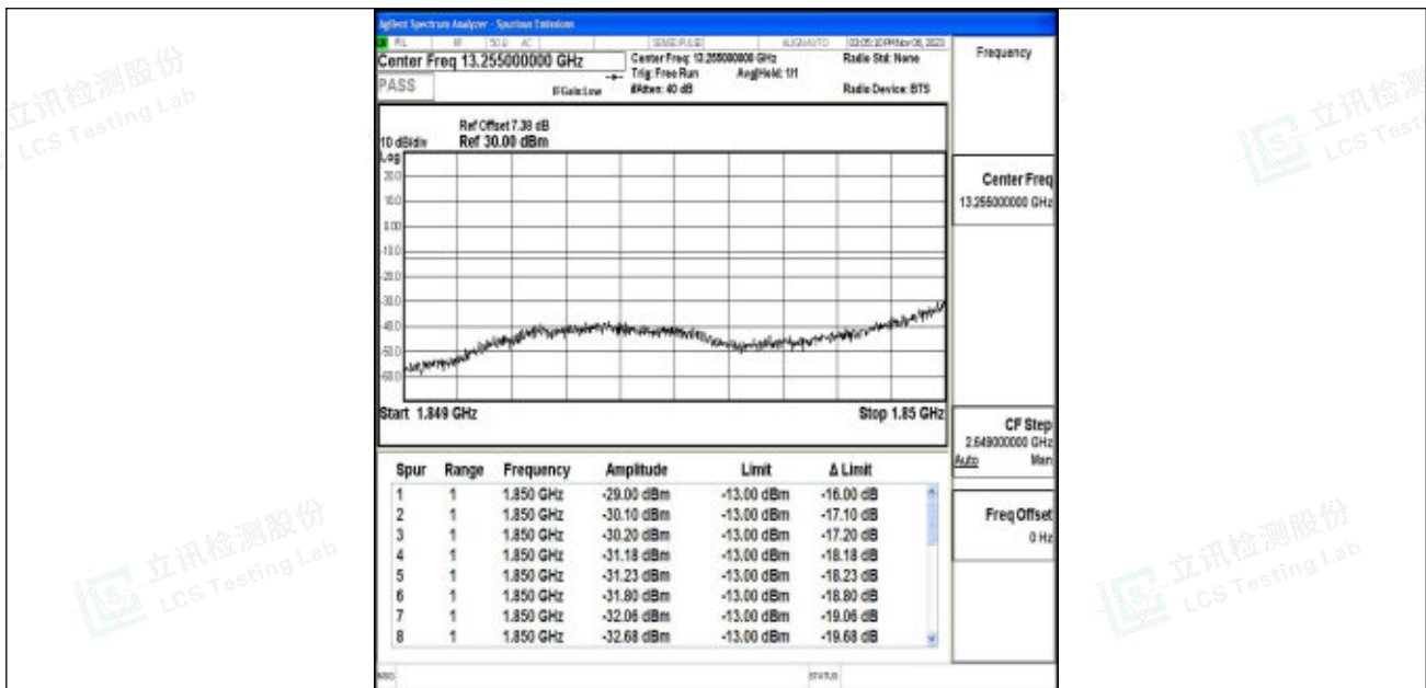
Band2_1.4MHz_64QAM_18607_1RB#0
