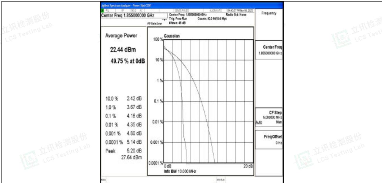
Band2-10MHz-64QAM-18650-1RB#0-PASS
