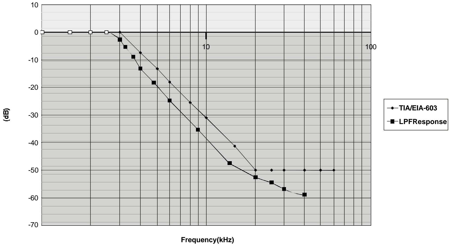
AudioLowPassFilterResponse
