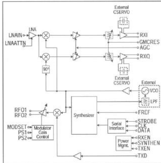
CT-D201 RF Block Diagram
