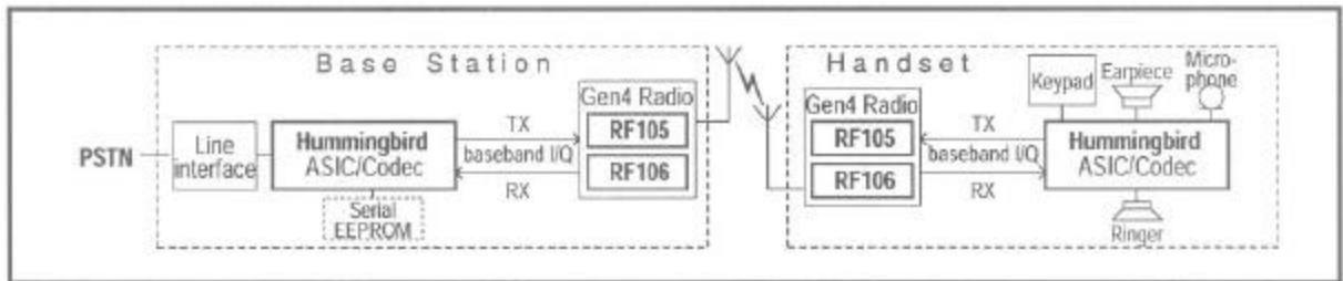
CT-D201 Spread Spectrum Telephone System Architecture
