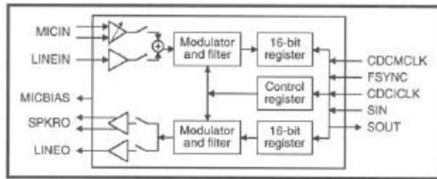
CT-D201 CODEC Block Diagram
