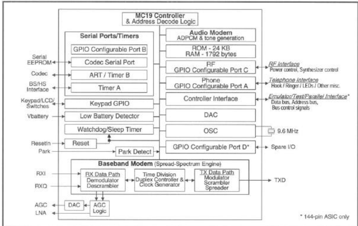
CT-D201 ASIC Block Diagram
