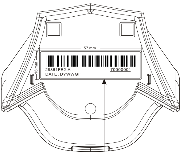
Charger bottom
