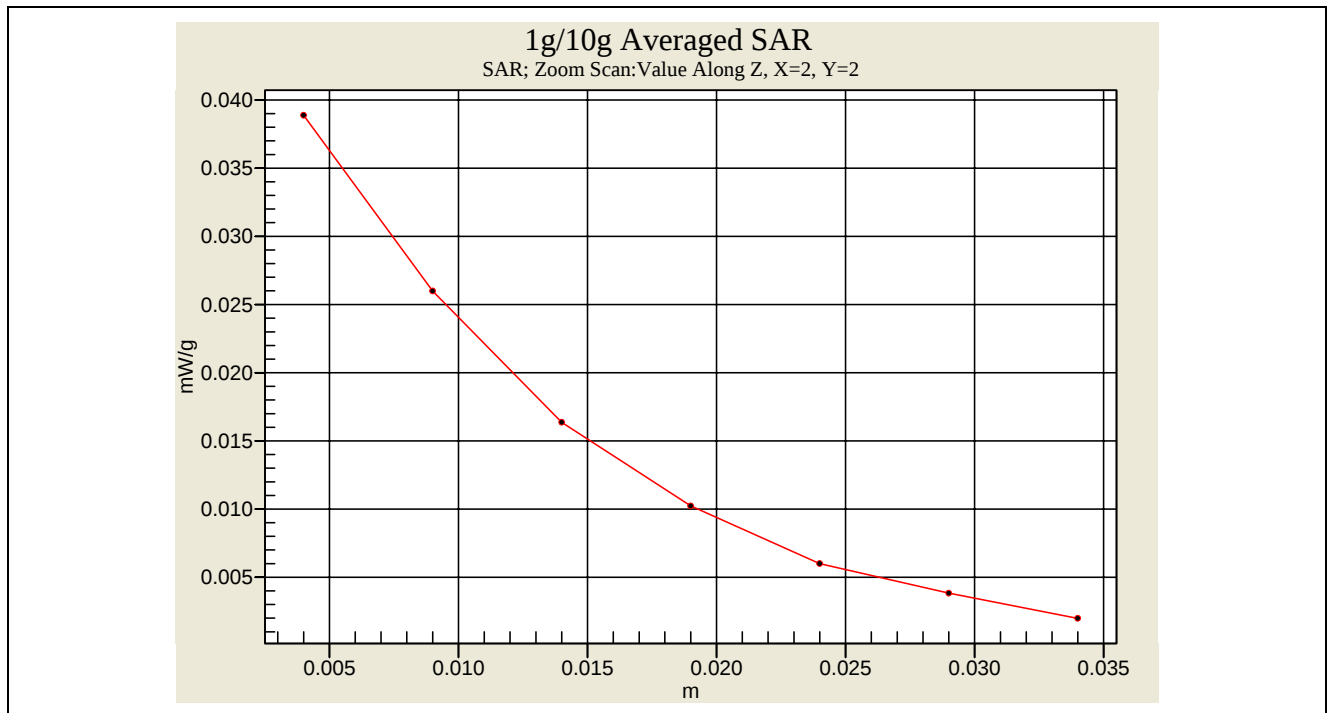
SAR Measurement _ Right Cheek CH4 (Ni-MH battery)
