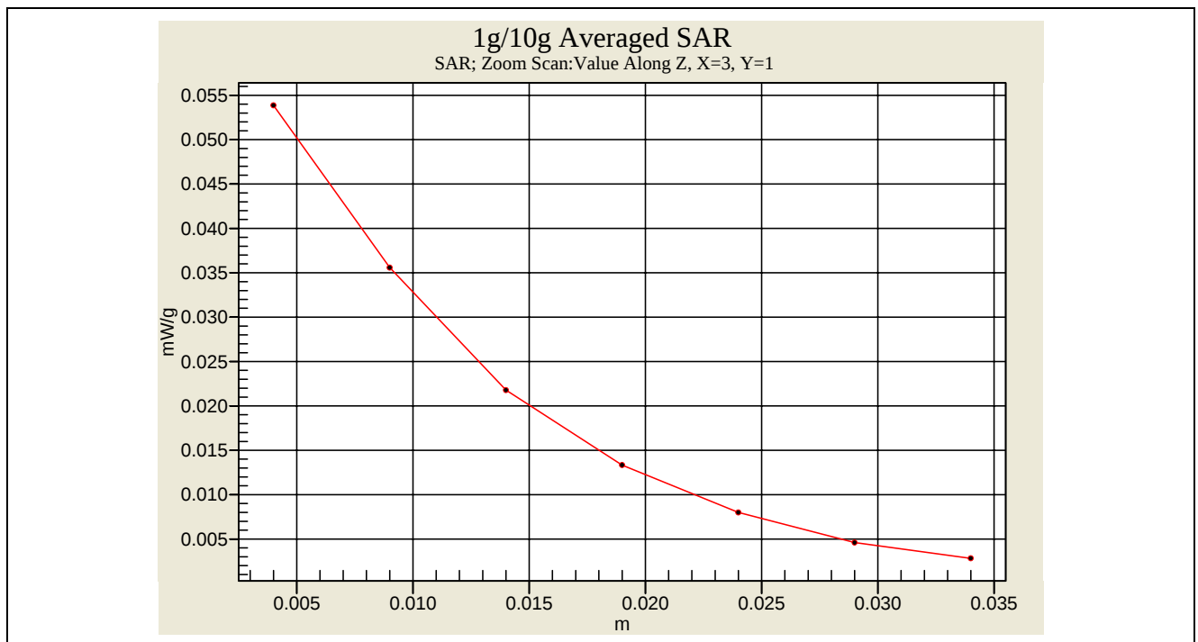
SAR Measurement _ Flat CH0 (Ni-MH battery)
