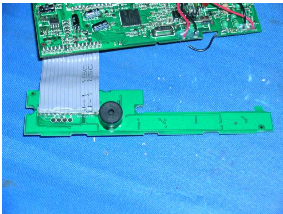
Base Unit Page Key front side (View 1)
