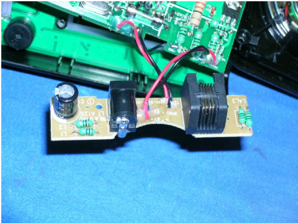
Base Unit AC Jack and Telephone Port front side
