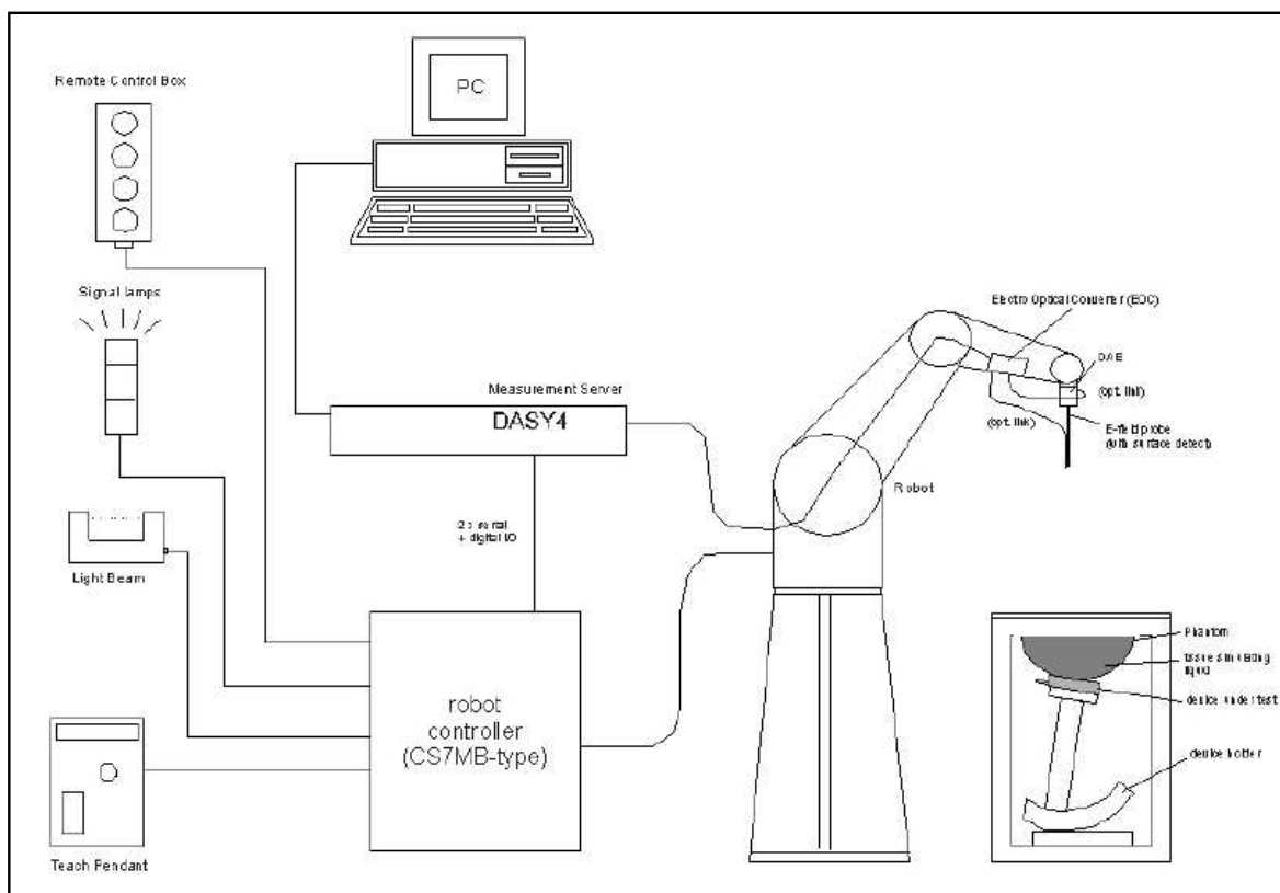
Fig. 5 The DASY4 Measurement System
