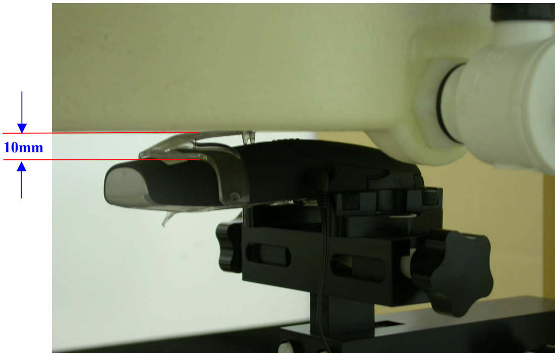
Measurement Position of Rear-UP with Handset
