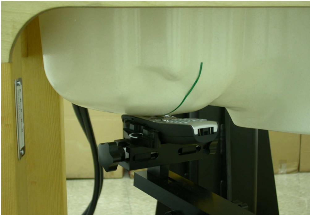
Measurement Position of Right-Cheek (RC) with Handset
