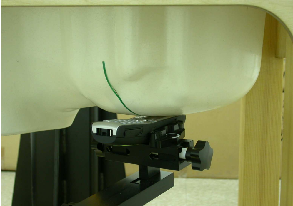
Measurement Position of Left-Cheek (LC) with Handset
