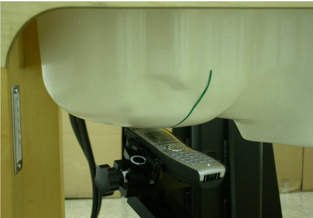
Measurement Position of Right-Tilt (RT) with Handset
