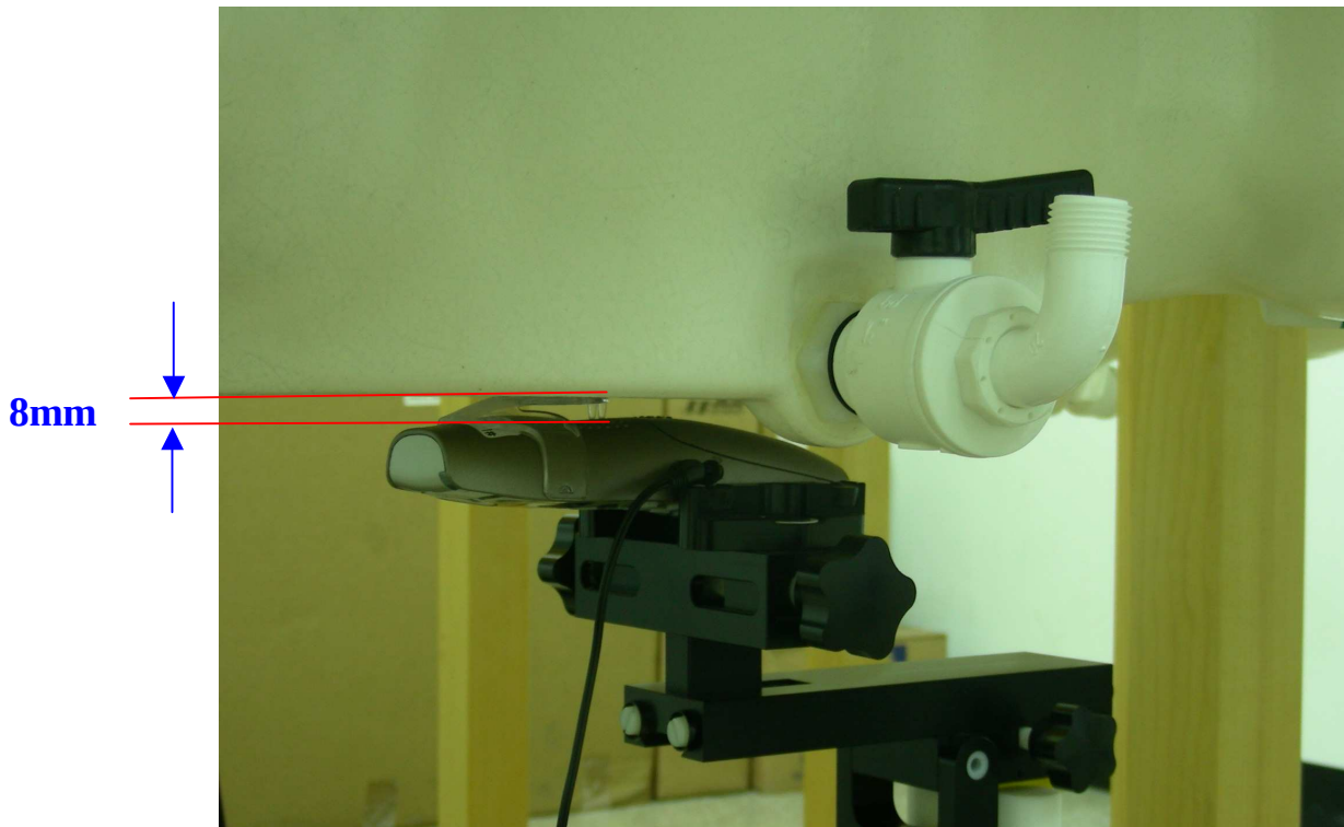
Measurement Position of Rear-UP with Handset Belt-Clip
