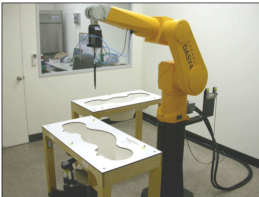
Fig. 6 The DASY4 System used in ETC set-up with two phantoms
