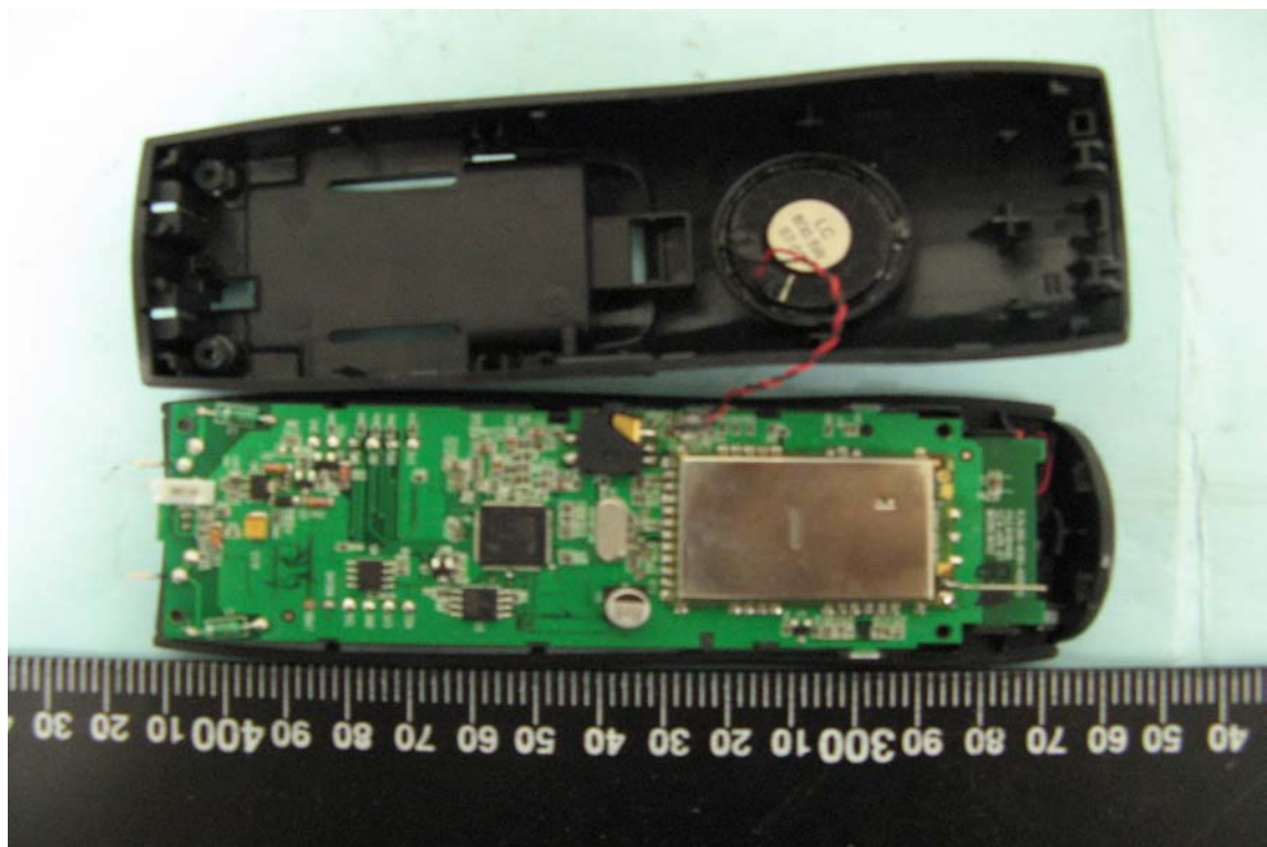
Internal View of Handset
