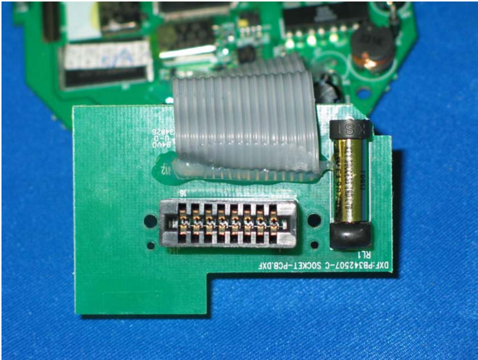
Docking Station connector PCB front side (View 1)
