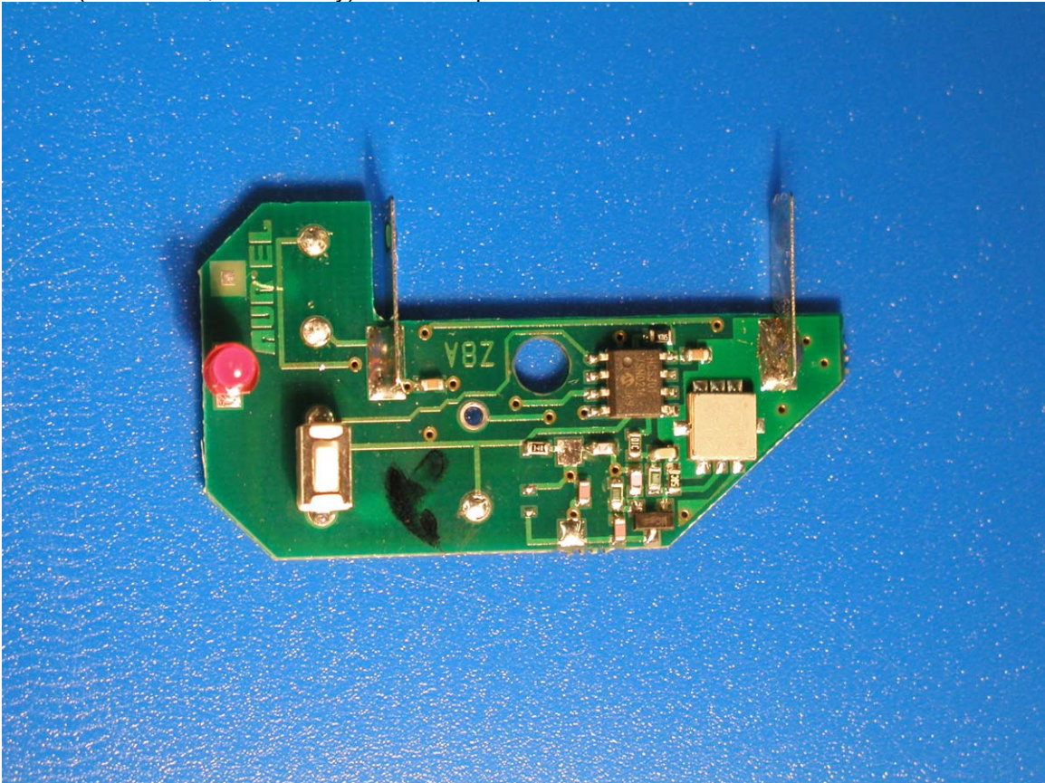
Transmitter #1 (Standalone, 12V Battery) - Board Bottom
