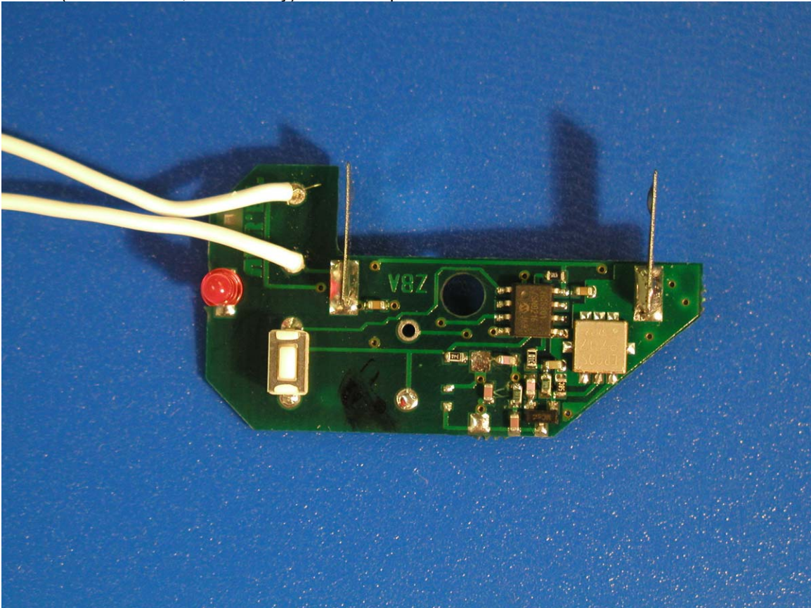
Transmitter #2 (external wires, 12V Battery) - Board Bottom
