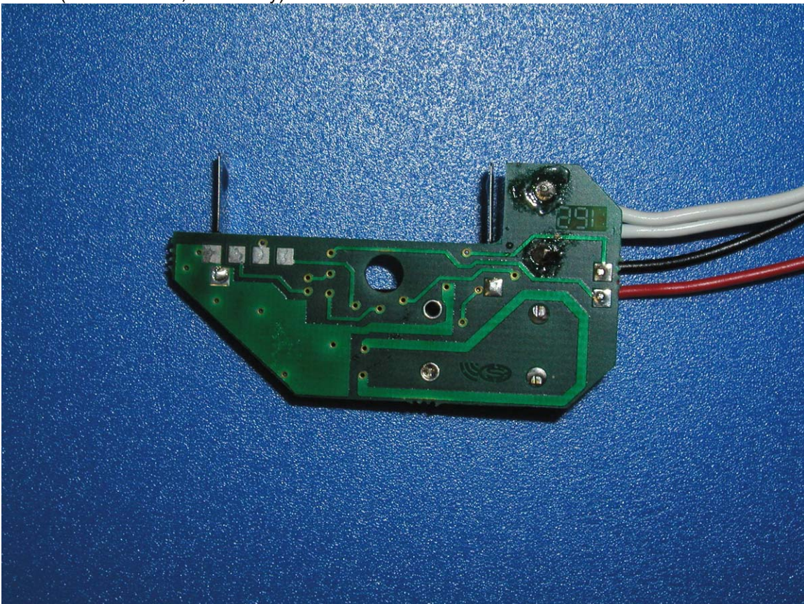
Transmitter #3 (external wires, 9V Battery) - Board Bottom
