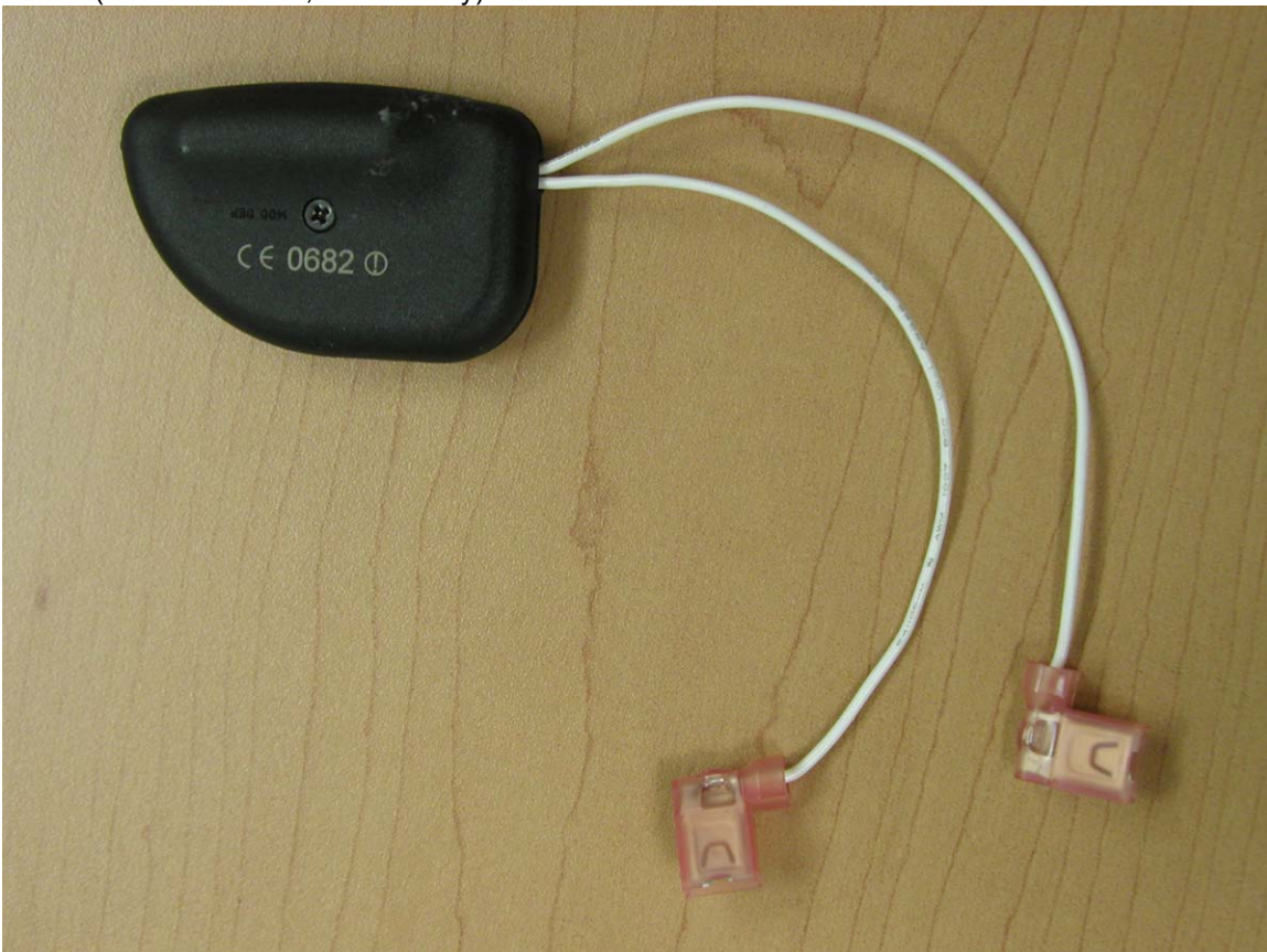
Transmitter #2 (External cables, 12V Battery) - Bottom
