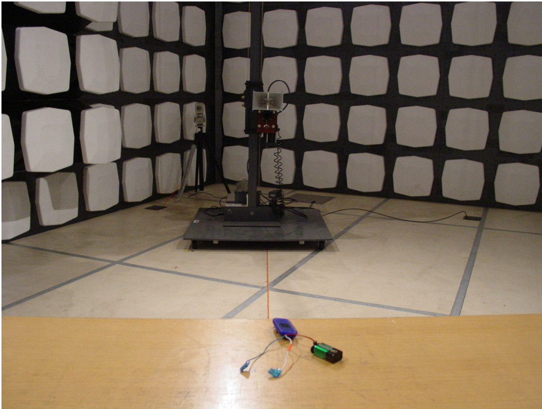
1GHz – 7GHz Vertical
