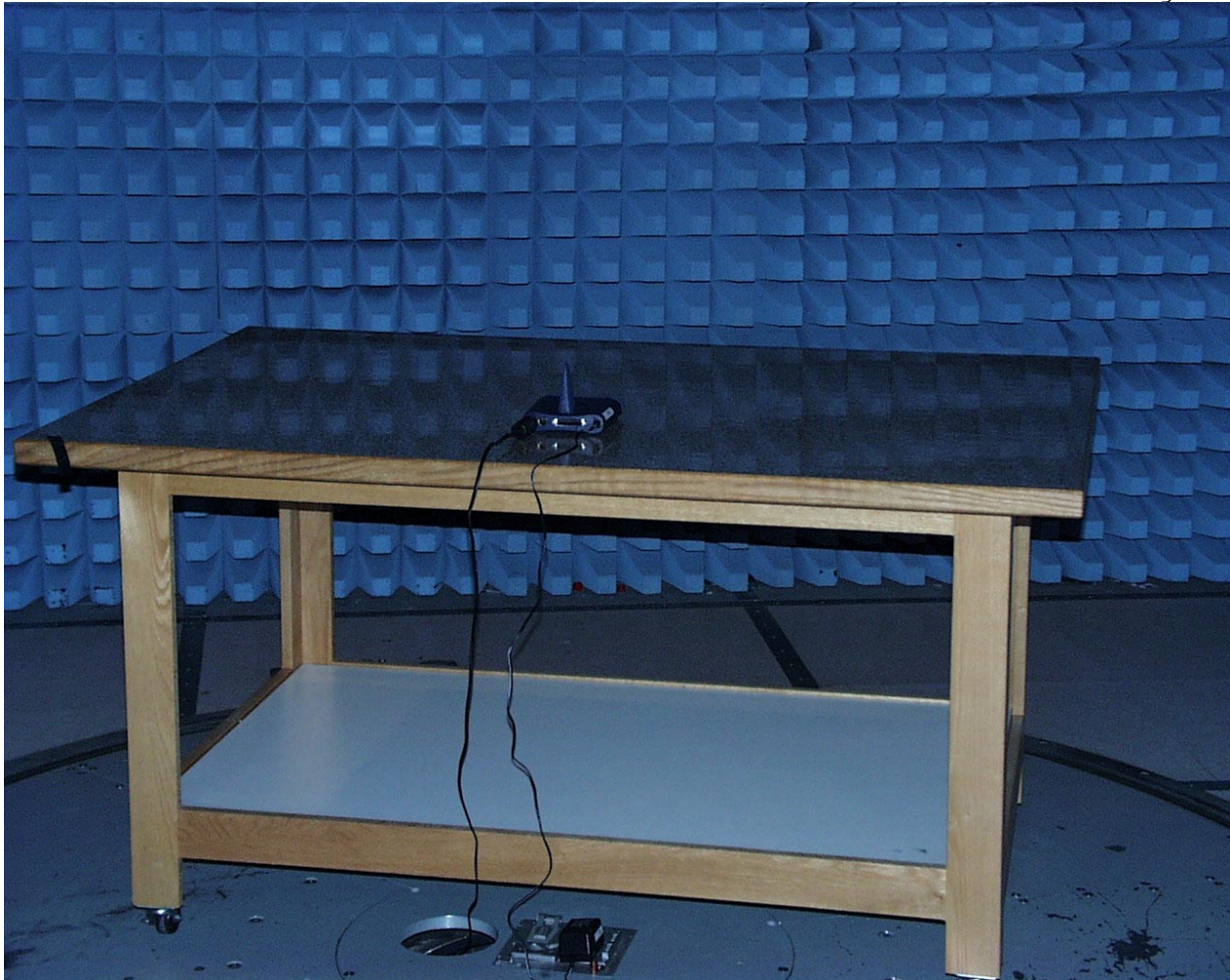
Back View of Worst Case Radiated and Line Conducted Emissions Test Set-up
