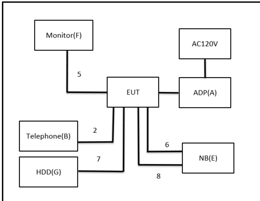
Radiated Emissions
