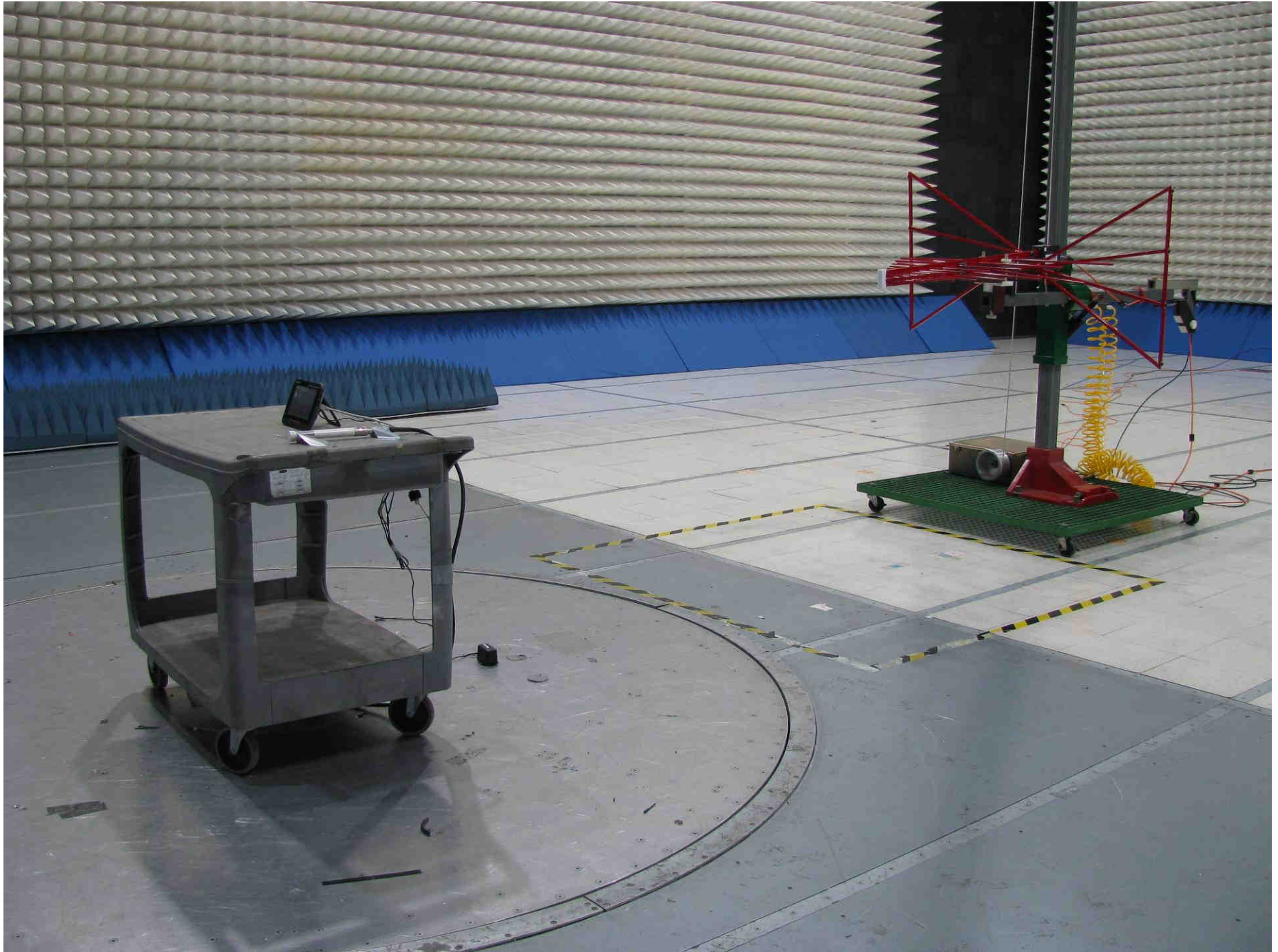
Radiated Bilog
