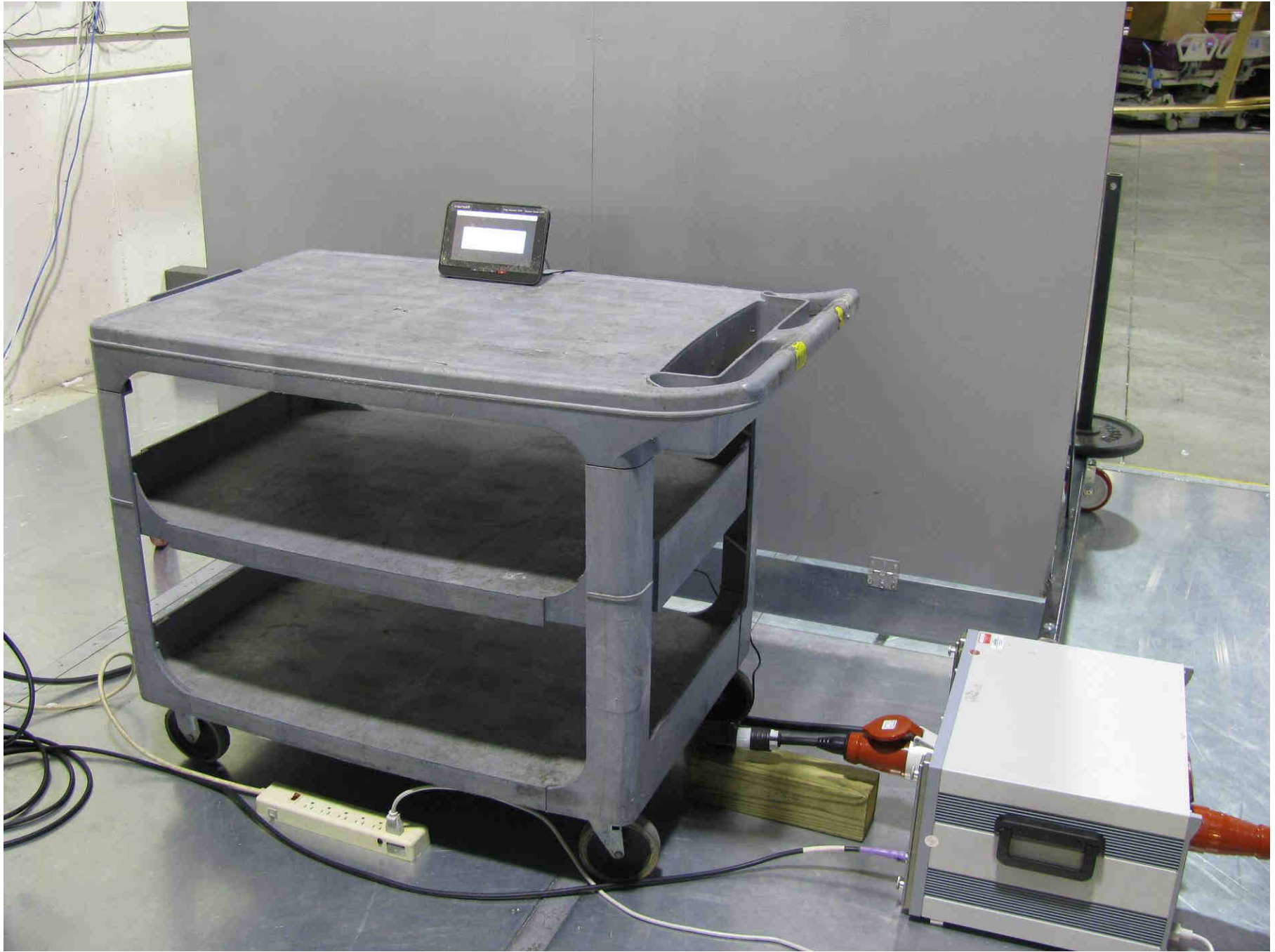
Conducted Emissions
