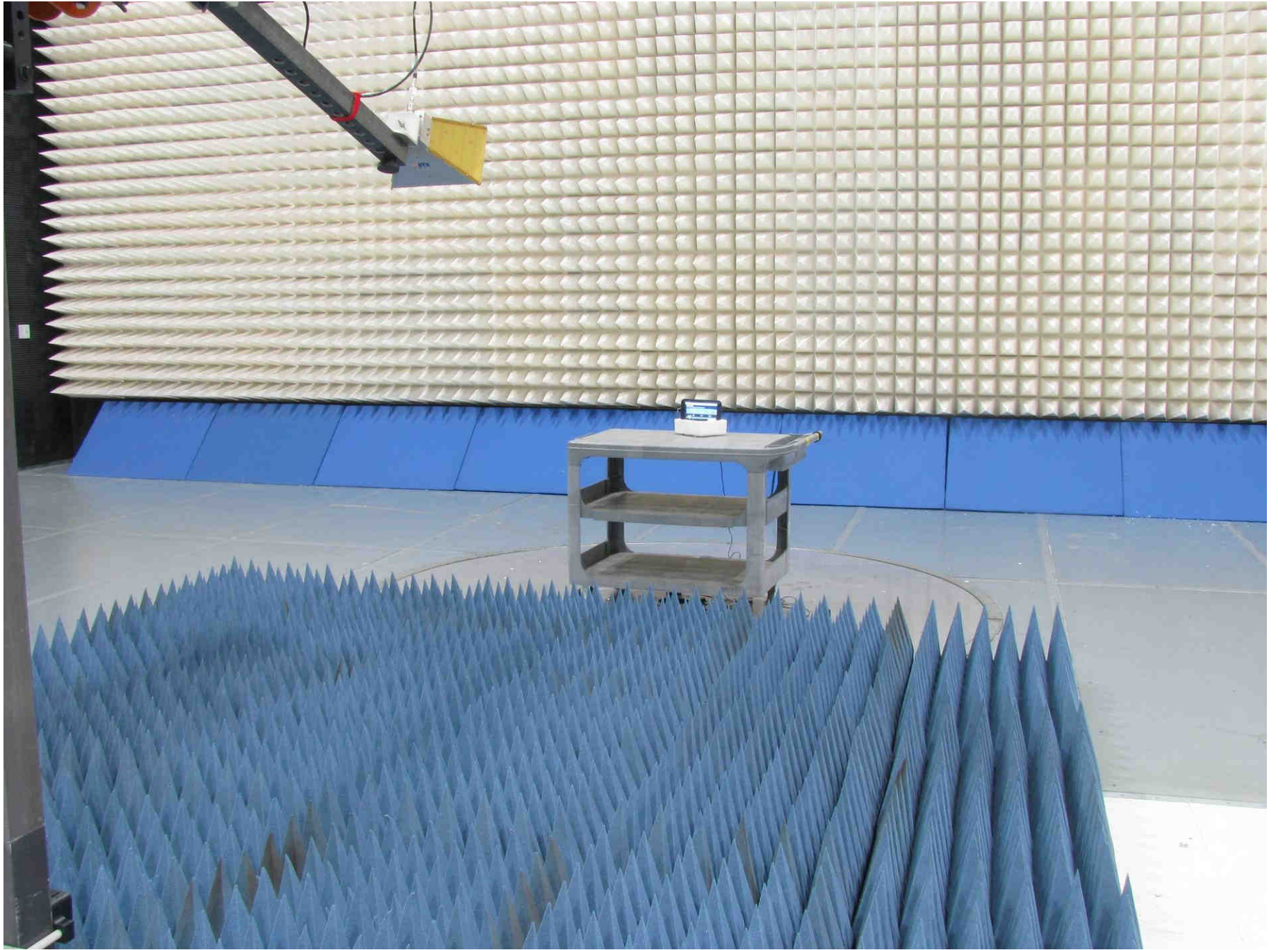
Radiated Horn
