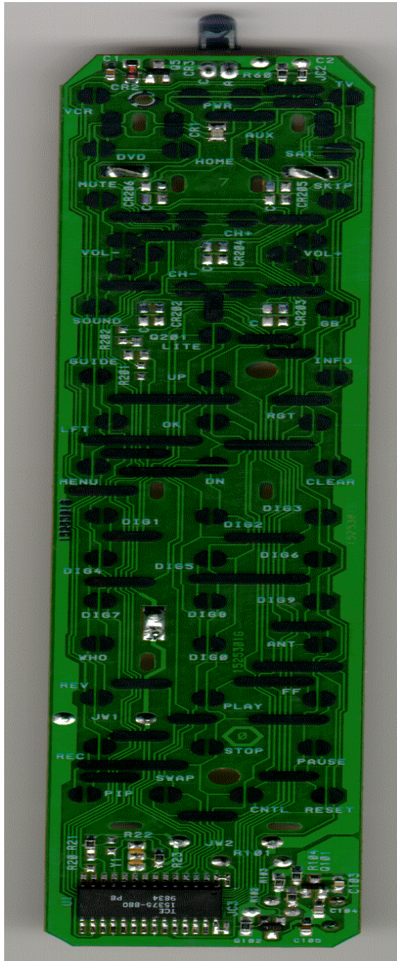
Component Side of the CRK 76
