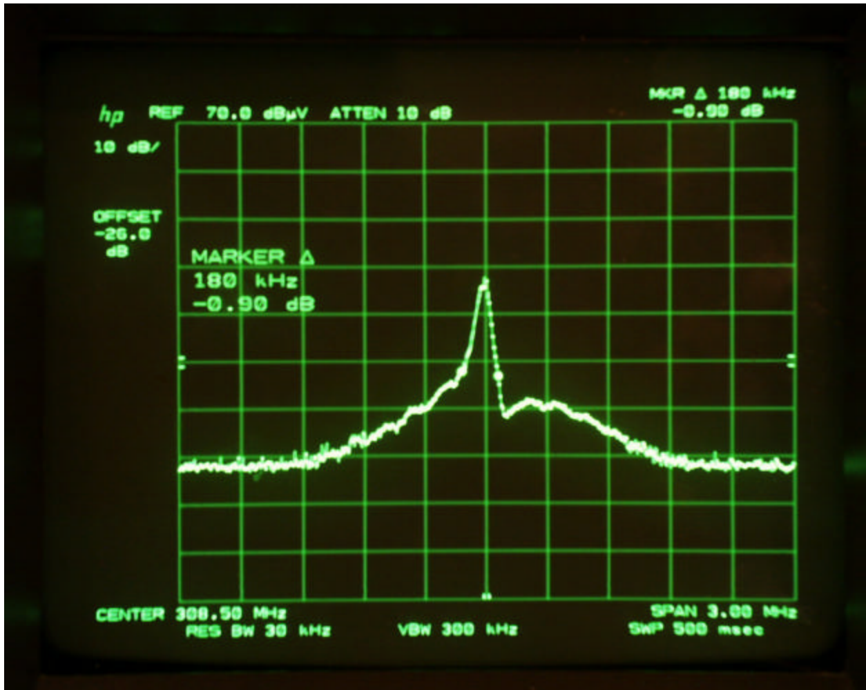
Plot 3 - Emission Bandwidth
