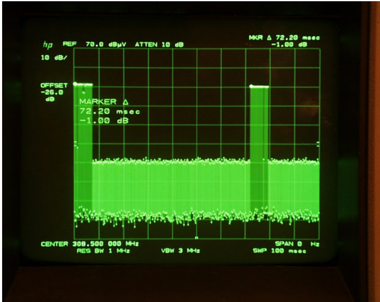
Plot 2 - Pulse Train Plot (100 msec)
