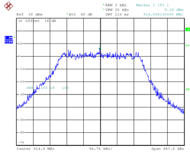
914.9MHz
