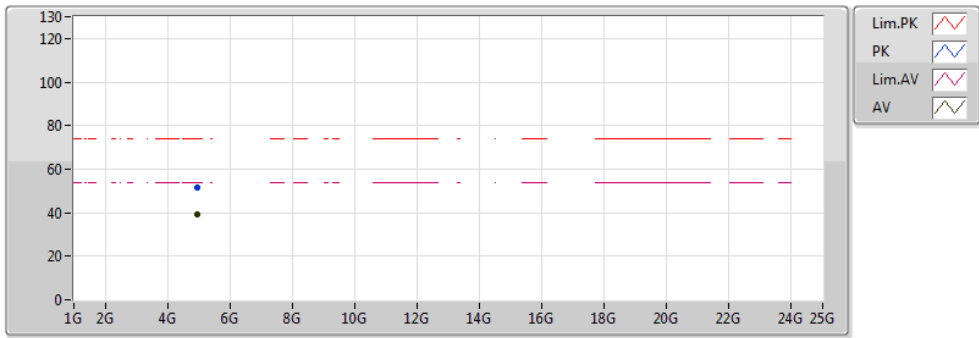
RE TX above 1GHz;Band:2.4G;Zigbee;BWch:5MHz;Nss:1;Nant:1;Ch:2475MHz;TX
