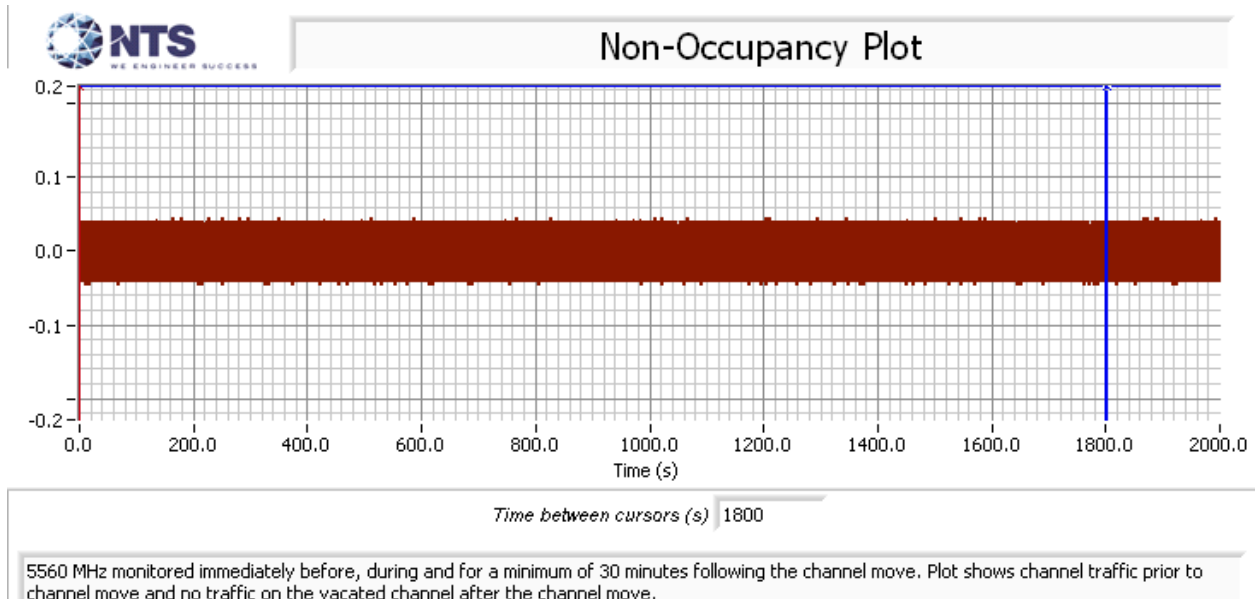
Figure 12 Radar Channel Non-occupancy Plot
