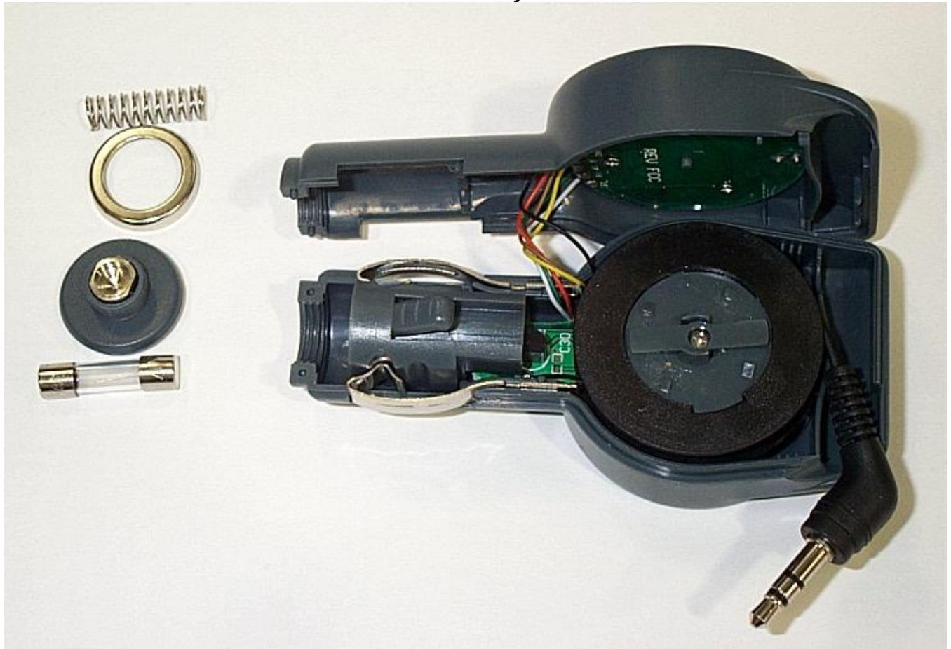
Inside of EUT Partially disassembled
