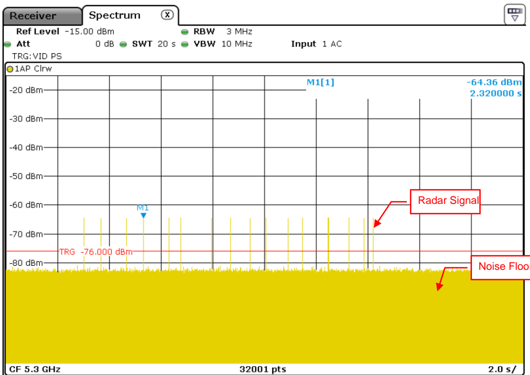
Radar Signal 5
