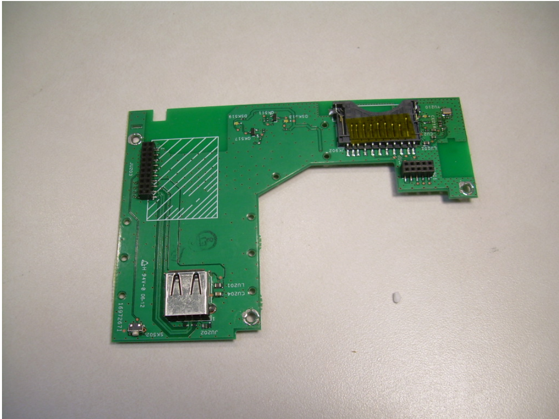
Photograph 15 – Bottom View of the Daughter Card with the 802.11abgn Module Removed
