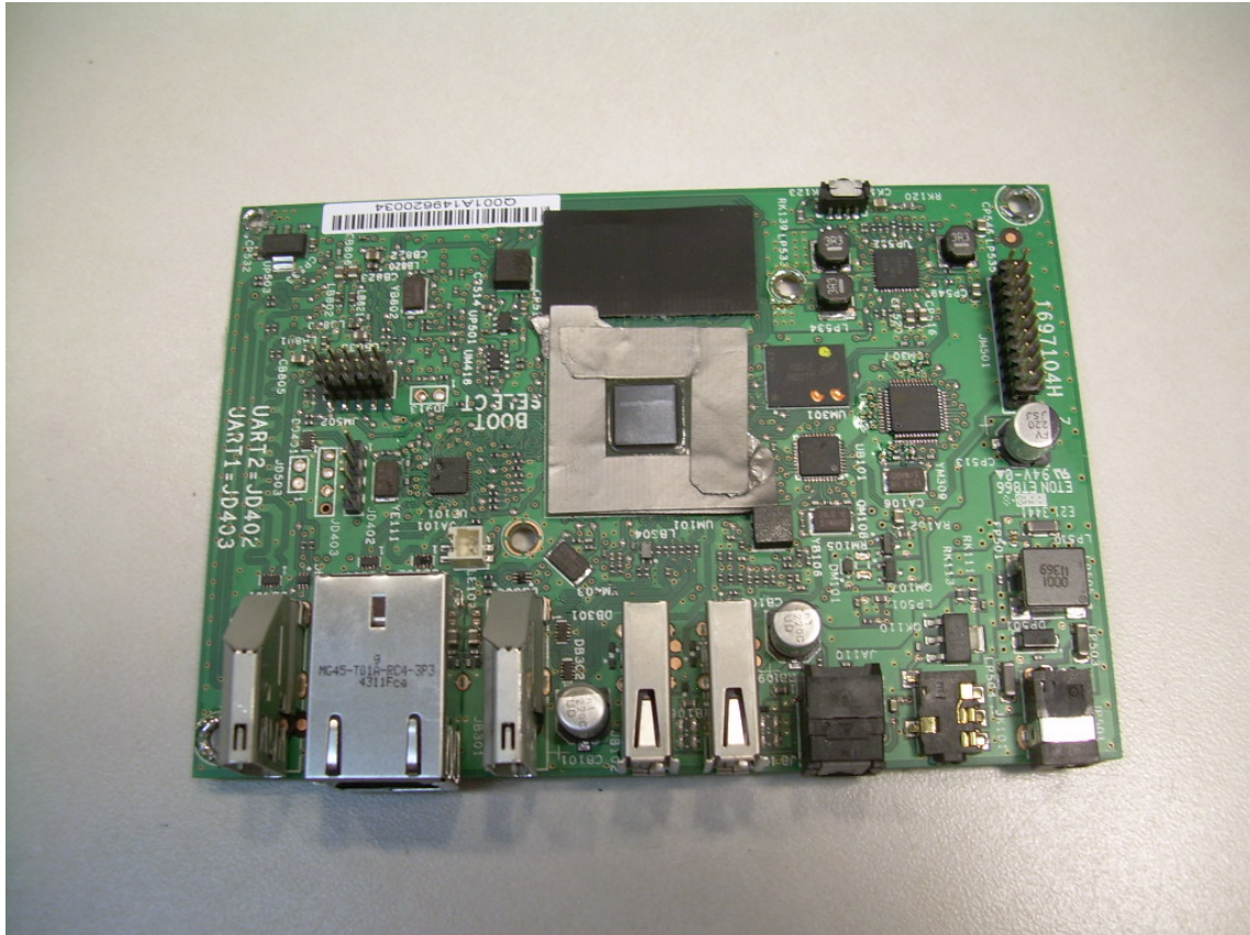
Photograph 11 – Top View of the Main PCB with Heatsink Removed
