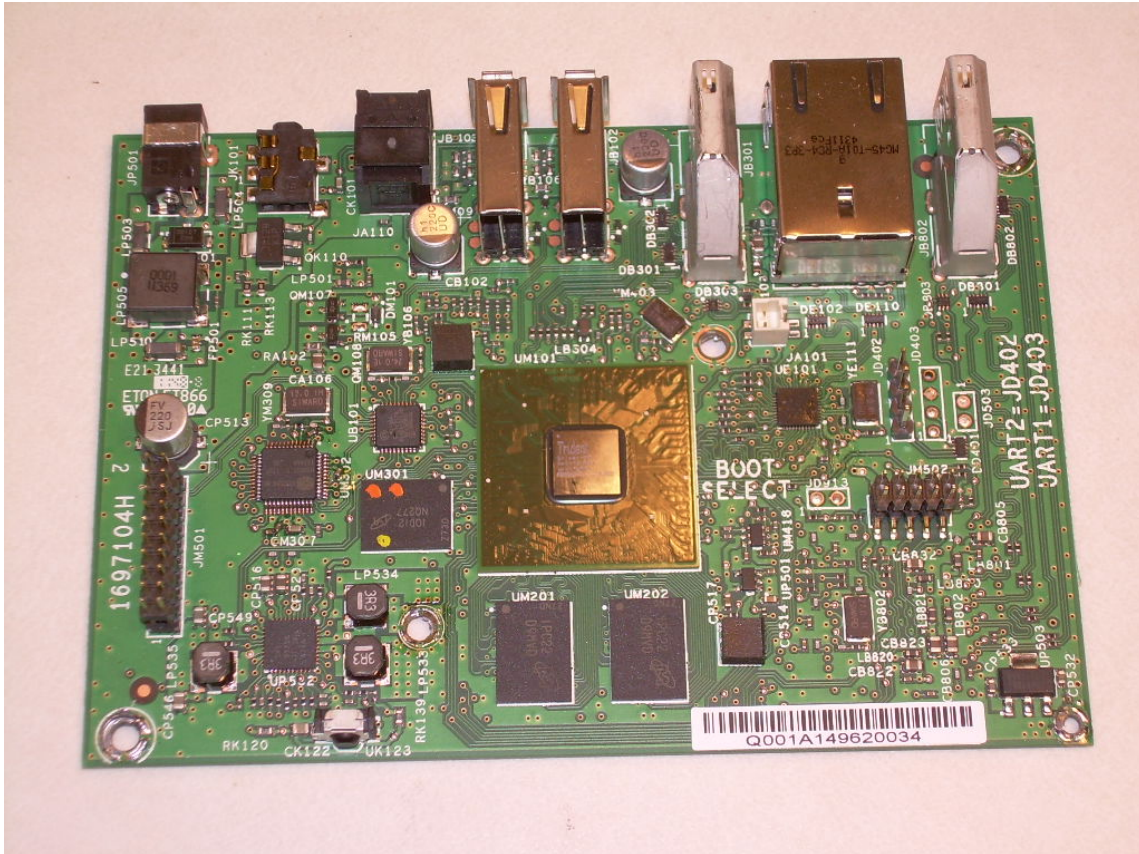
Photograph 12 – Top View of the Main PCB with RF Absorber Removed
