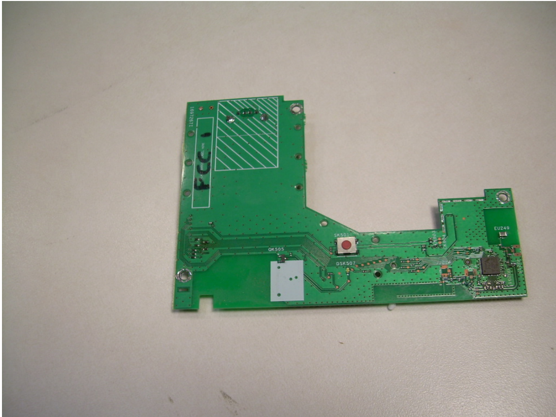
Photograph 16 – Top View of the Daughter Card
