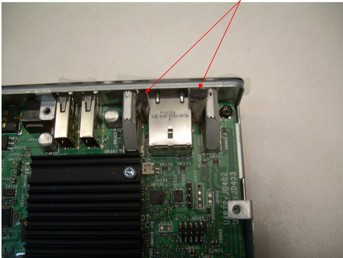
Photograph 9 – View of the Connector Gasketing
