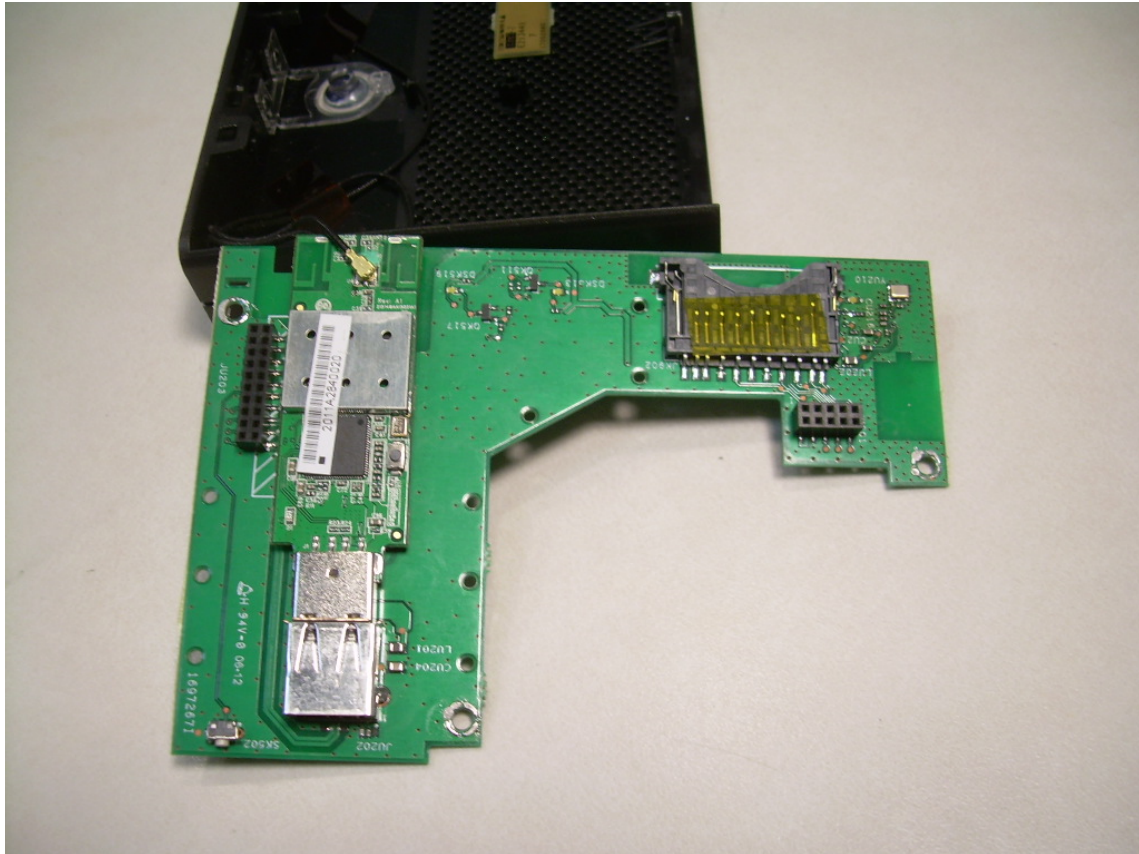
Photograph 14 – Bottom View of the Daughter Card with 802.11abgn Module Installed
