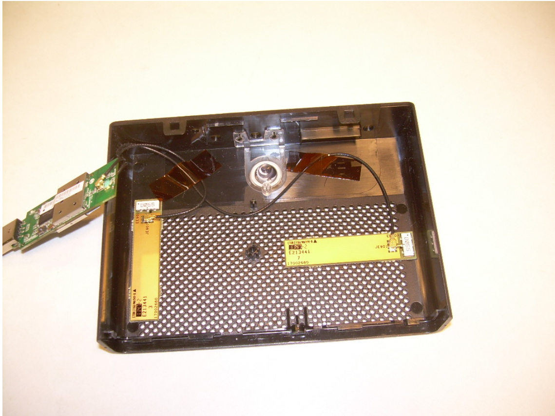
Photograph 17 – View of the Top Housing with the 802.11abgn Module and Antennas
