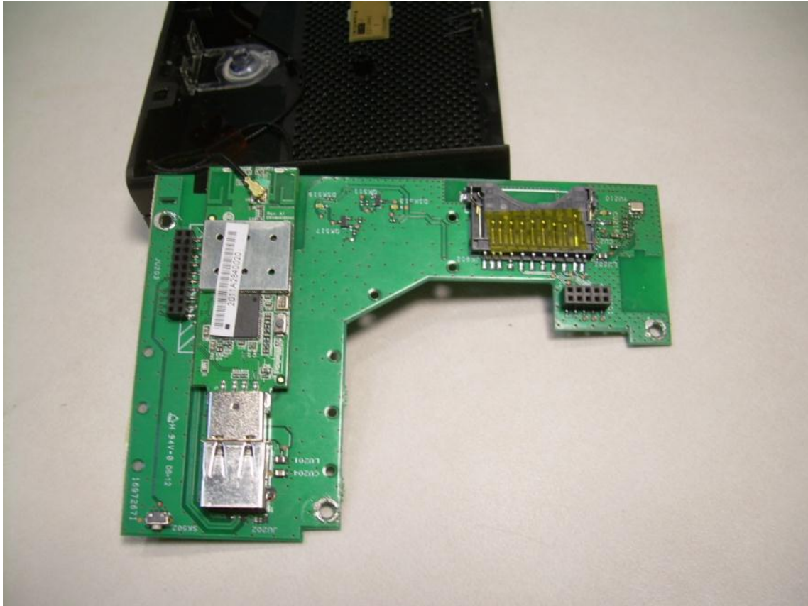
Bottom View of the Daughter Card with 802.11abgn Module Installed
