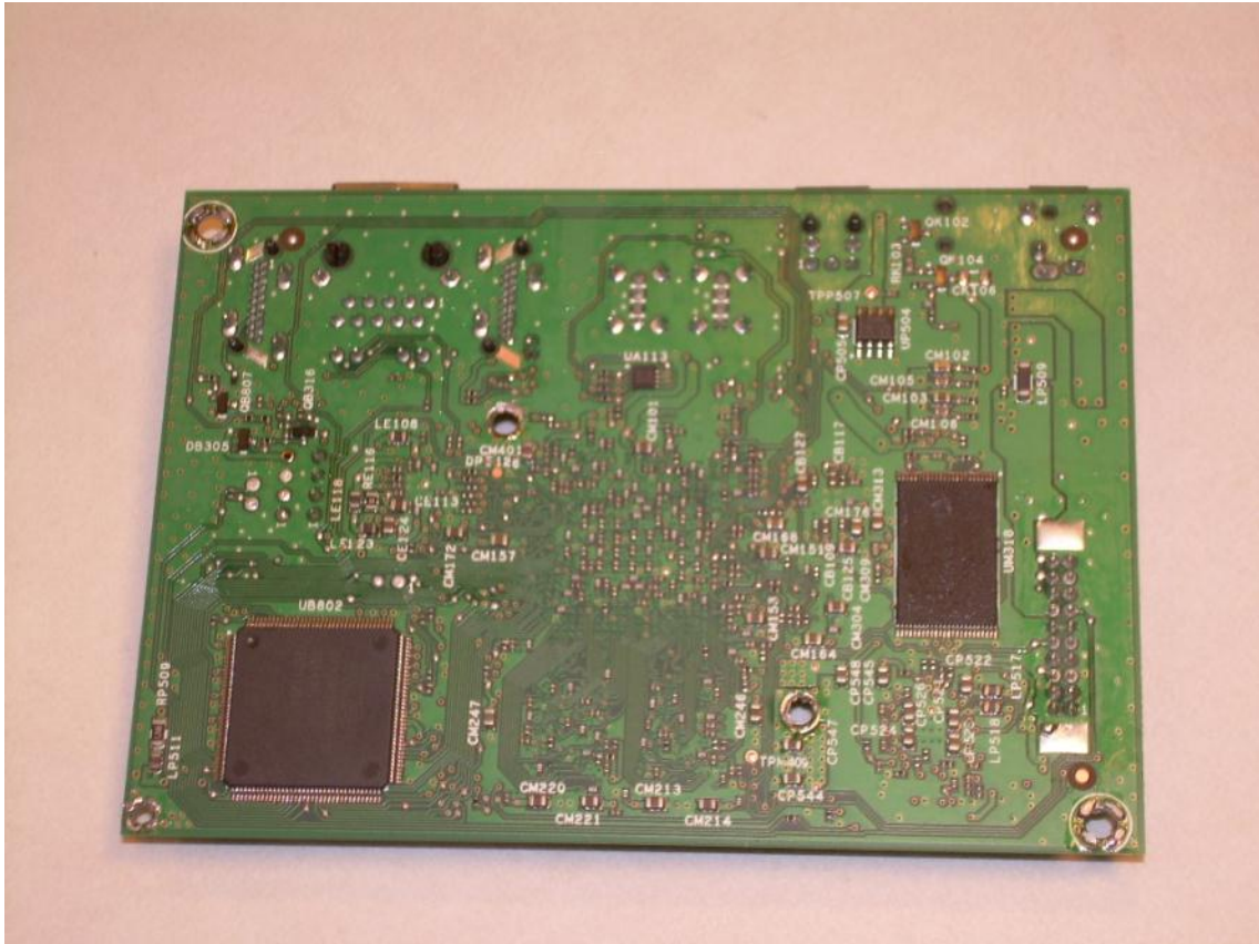
View of the Bottom Side of the Main PCB
