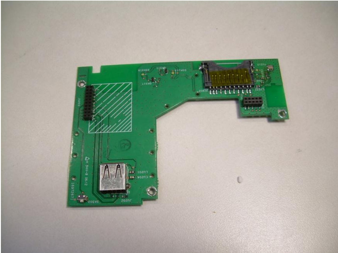
Bottom View of the Daughter Card with the 802.11abgn Module Removed
