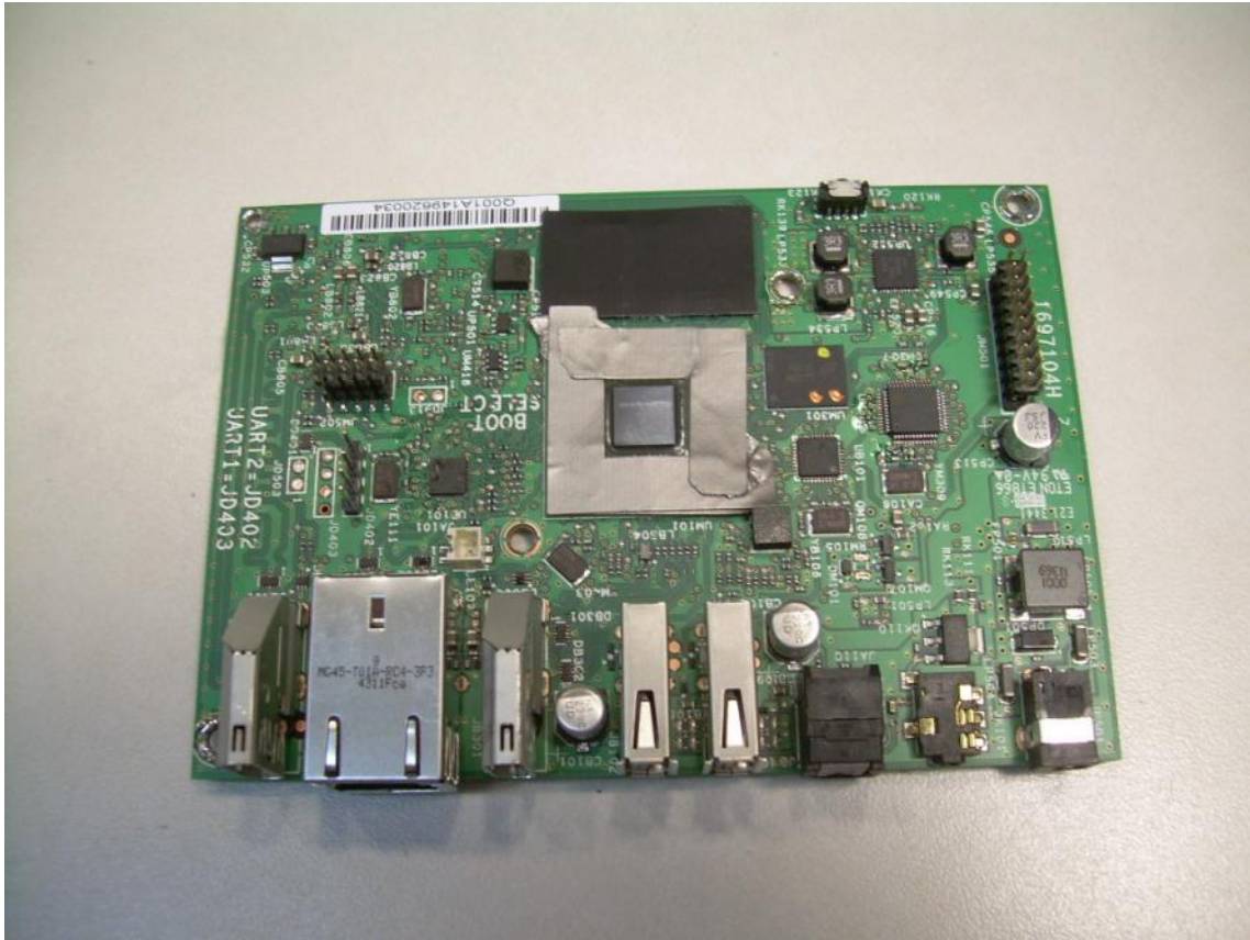
Top View of the Main PCB with Heatsink Removed
