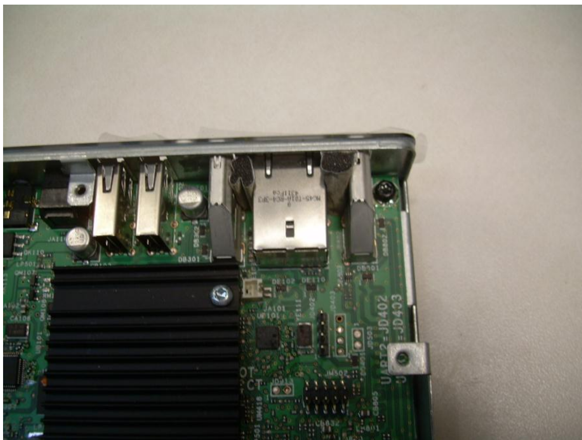
View of the Connector Gasketing
