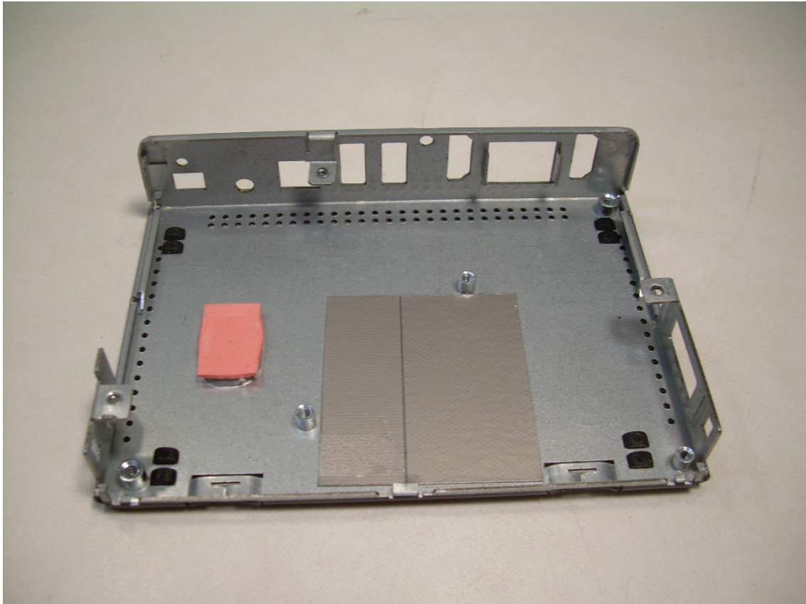
View of the Bottom Housing with RF Absorber
