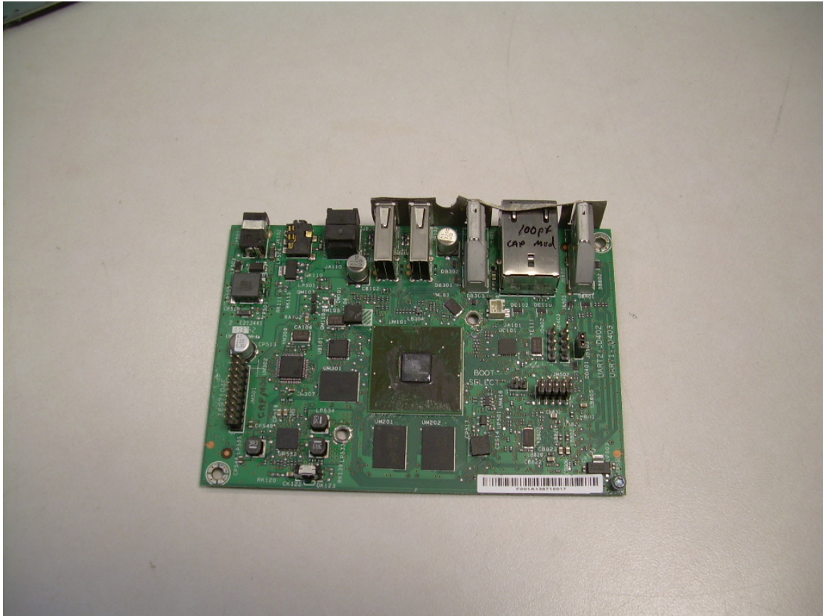
Top View of the Main PCB with RF Absorber Removed
