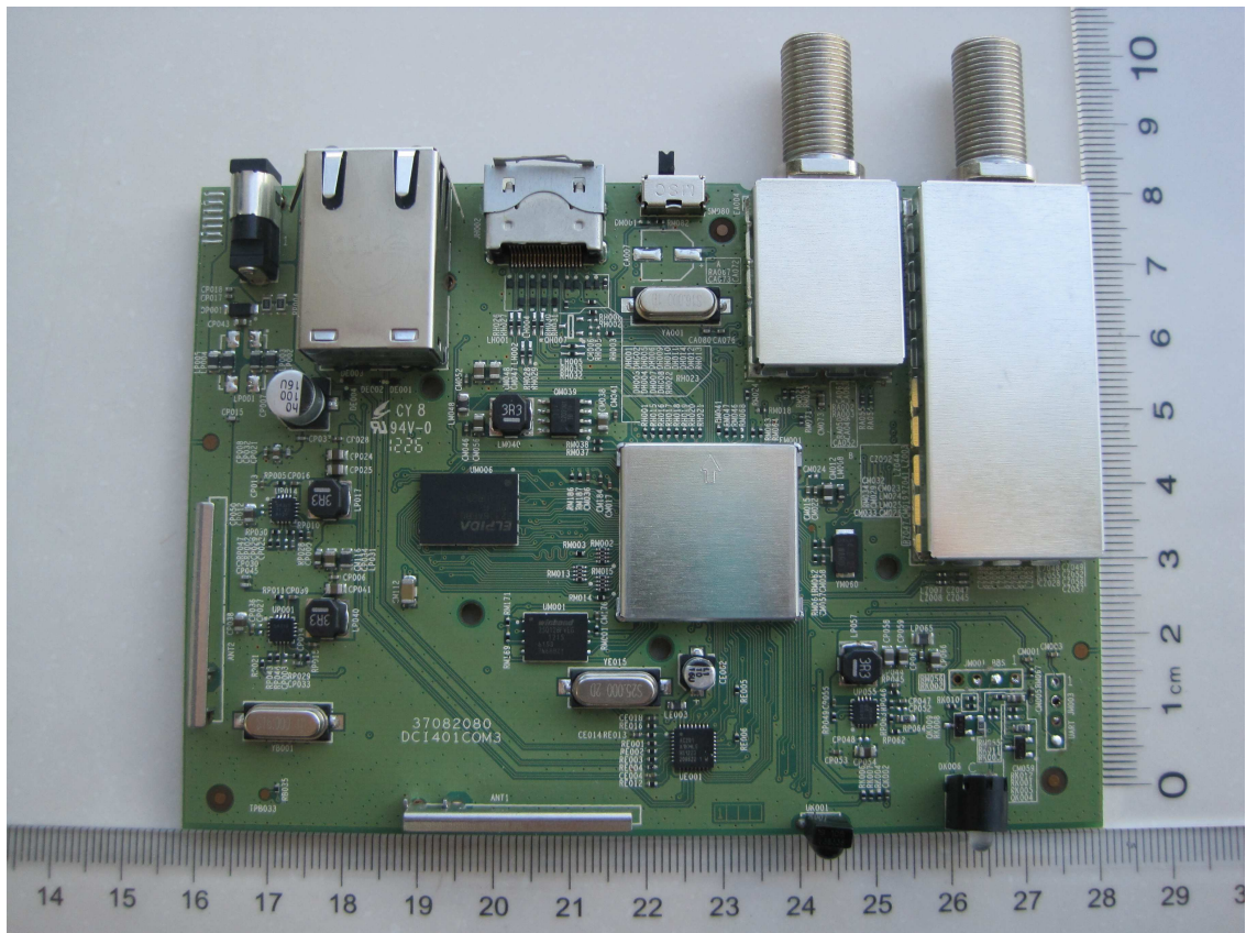
PCB top side-with shielding
