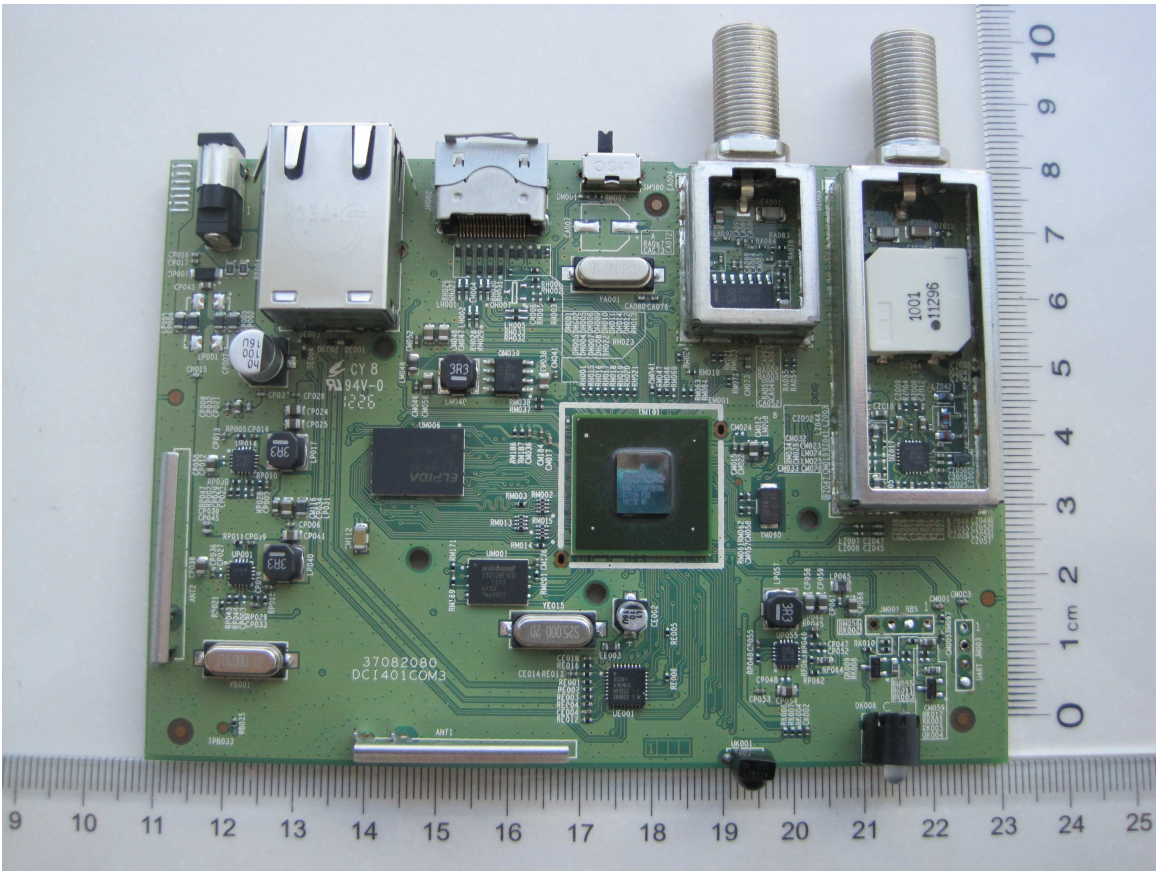
PCB top side-without shielding
