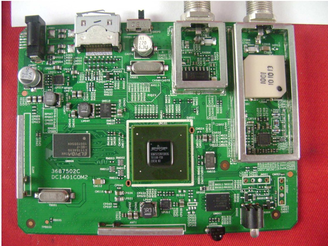
Pic5: PCB component side (without shielding) of DCI401GEU2
