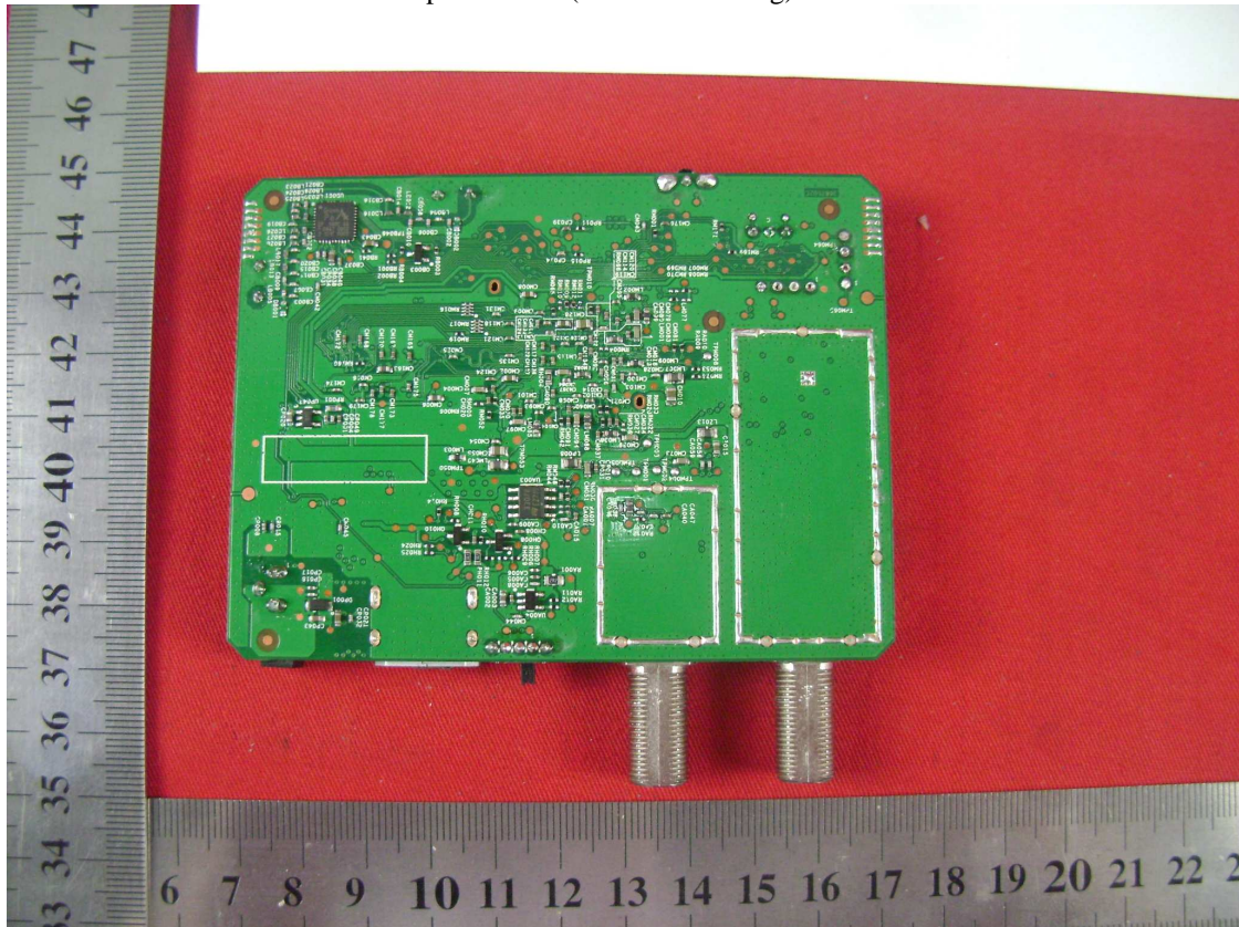
Pic6: PCB trace side of DCI401GEU2
