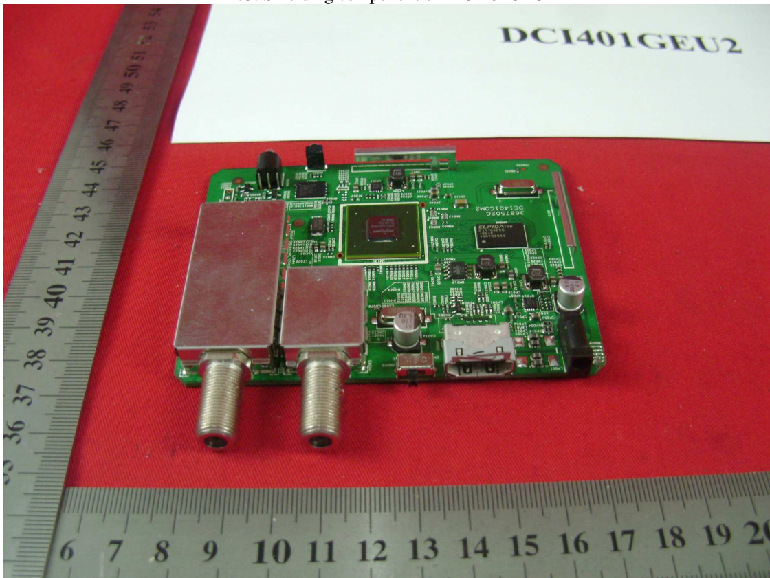
Pic4: PCB component side (with shielding) of DCI401GEU2
