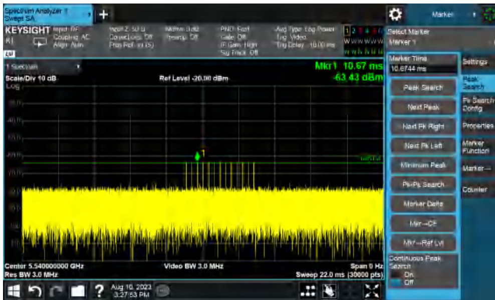
Radar Signal 4
