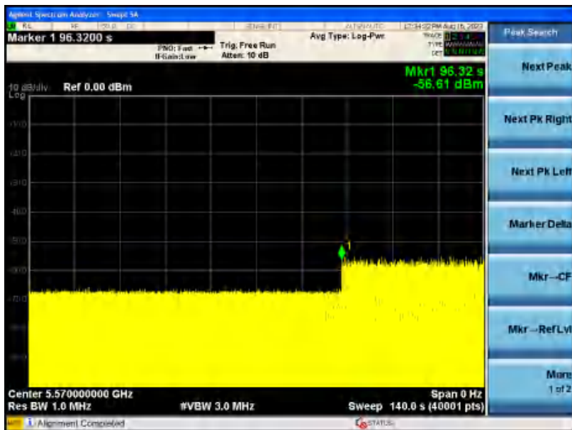
Initial Channel Availability Check Time: 96.32s
