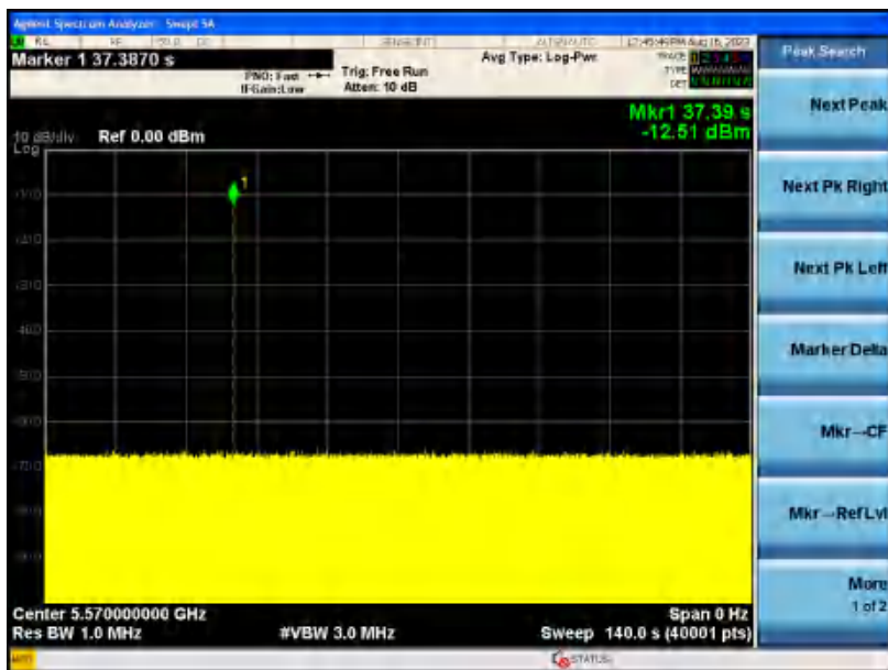
Inject radar signal at 37.39s
