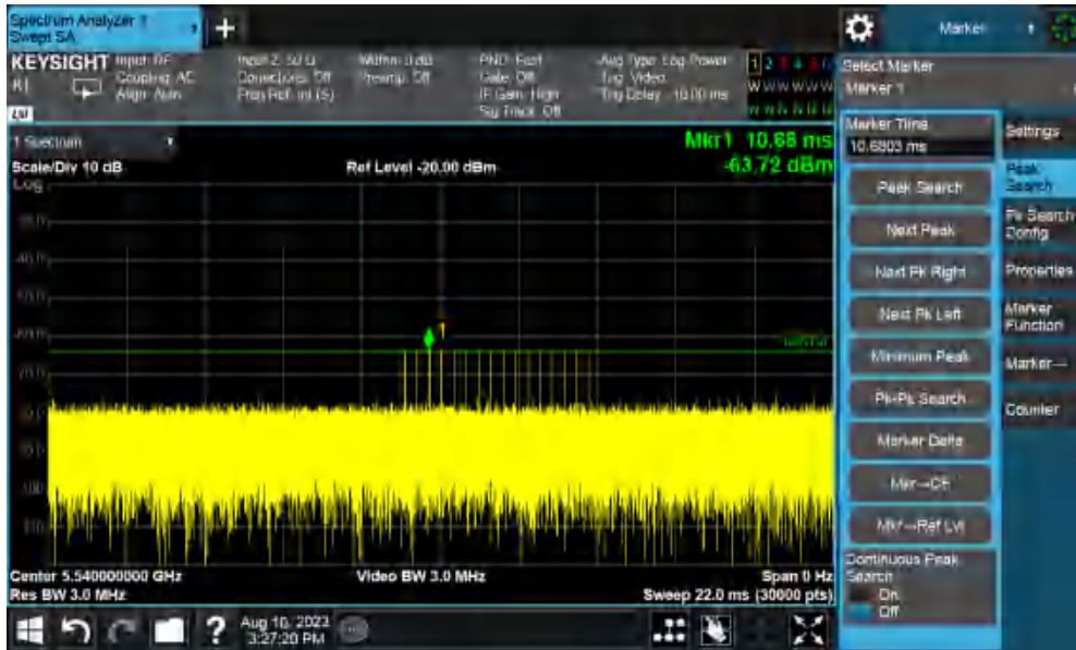
Radar Signal 4
