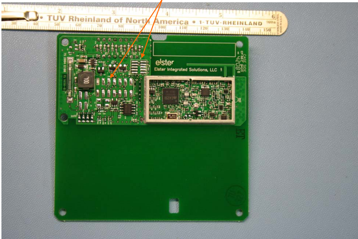
Photo of Production Model with RF shield removed
