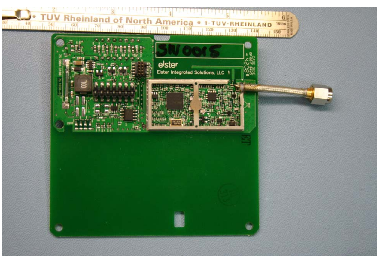
Photo of Test EUT with Coax attached for conducted measurements
