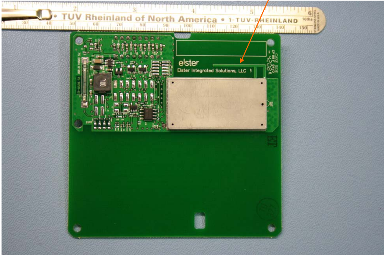
Front View Photo of Production module with RF shield
