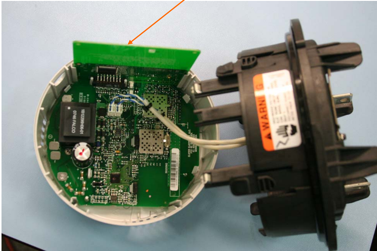
View of a Production Model installed in a “REX2” Power Meter (typical use for module)
