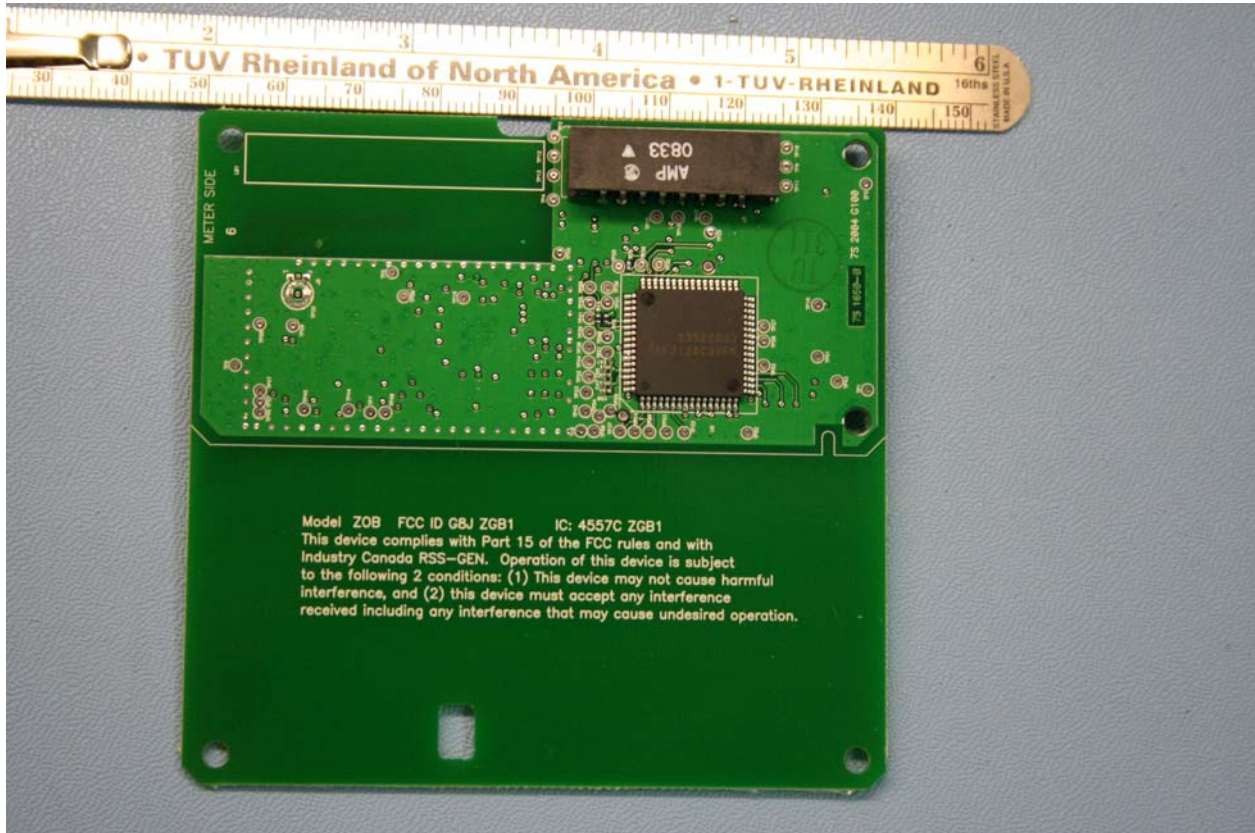
Rear View Photo of Production Model
