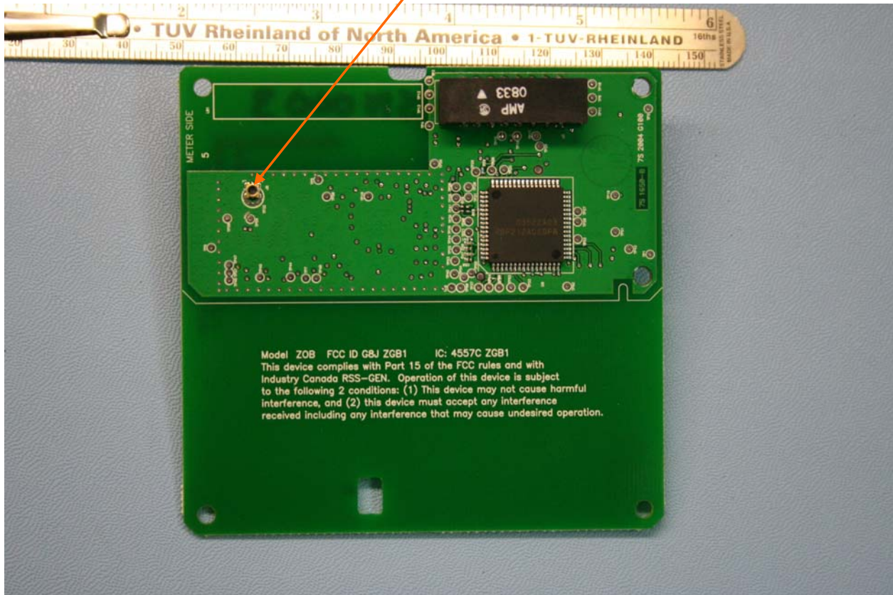
Rear View Photo of EUT
