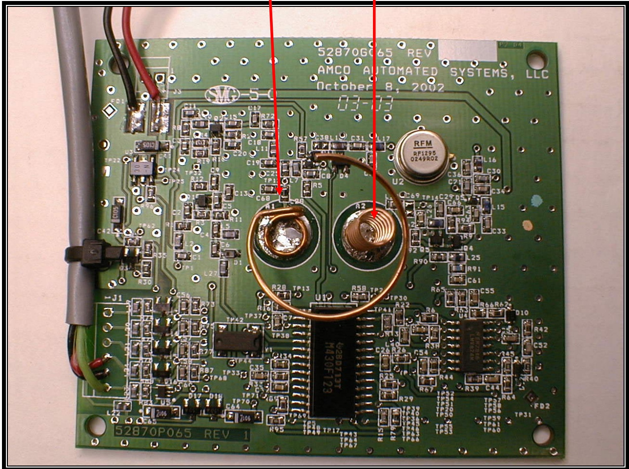
PHOTOGRAPH 1: ANTENNA LOCATION
