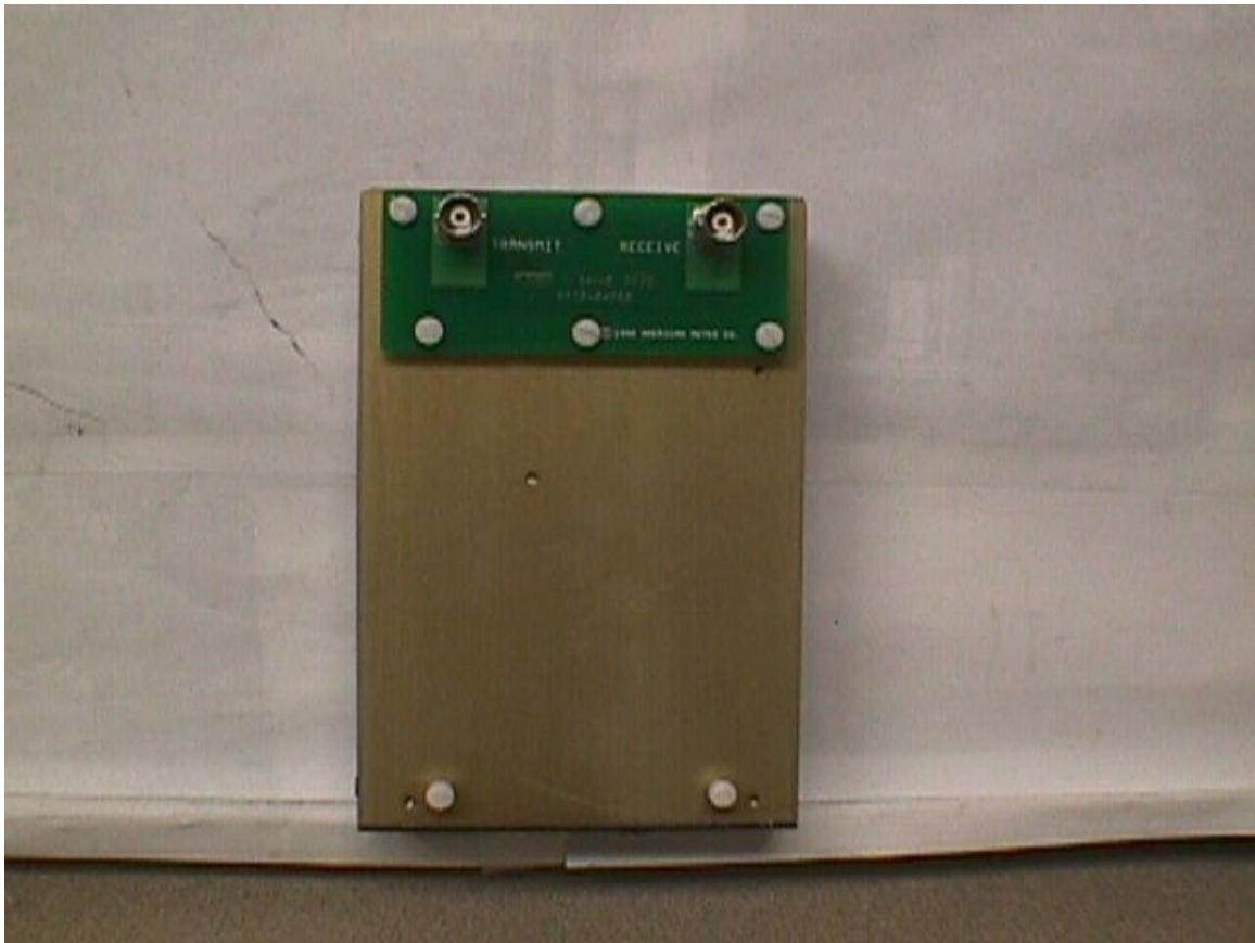
FIGURE 17: TRANSMITTER/RECEIVER BOARD
