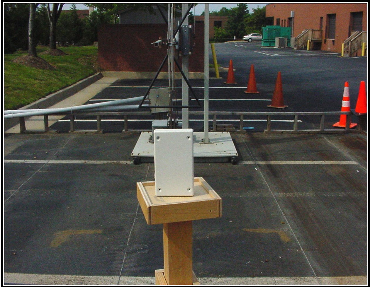
PHOTOGRAPH 4: RADIATED EMISSIONS REAR VIEW
