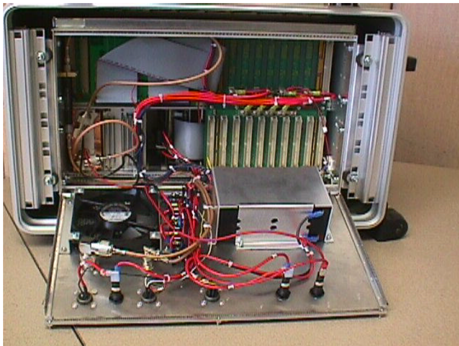
Figure 40: Back of EUT with cover open
