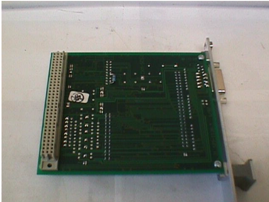
Figure 37: PEP Modular CXM SCSI, back
