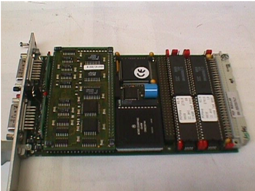
Figure 38: PEP Modular VM 30, front
