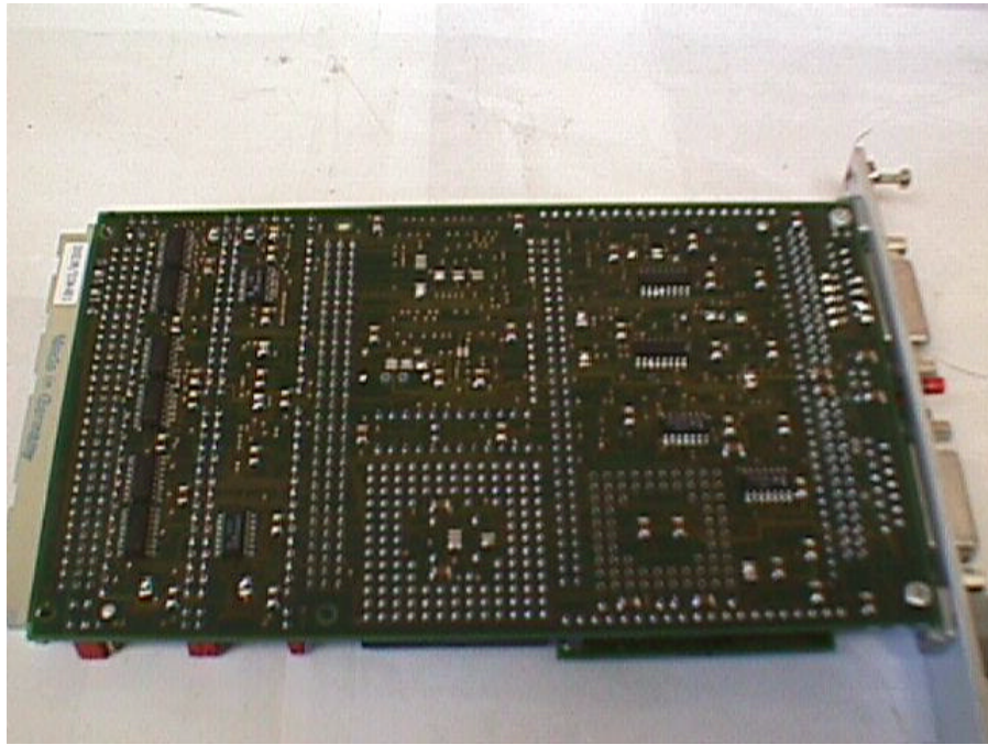
Figure 39: PEP Modular VM 30, back
