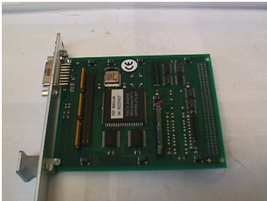
Figure 36: PEP Modular CXM SCSI, front
