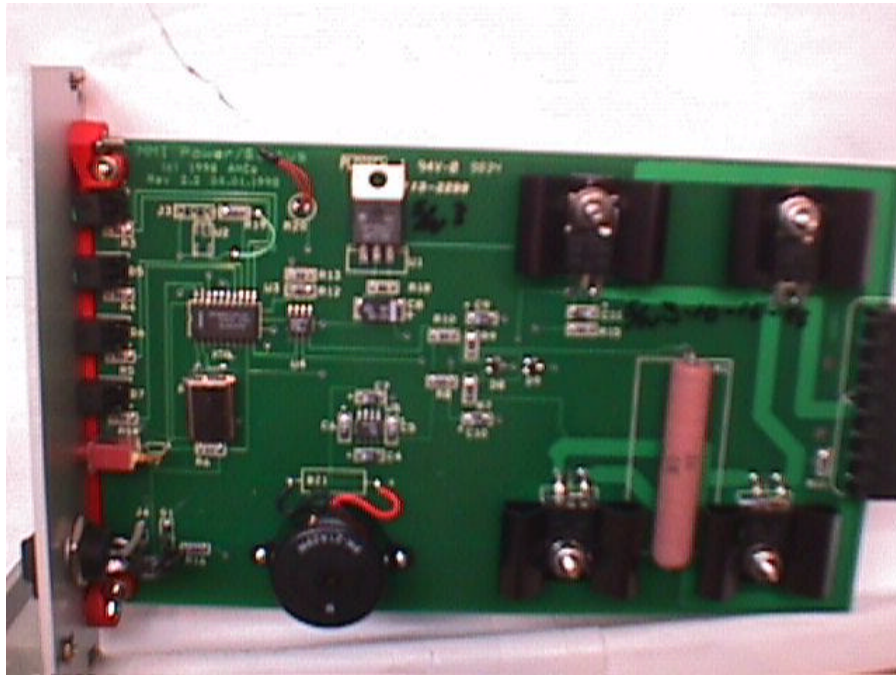
Figure 23: Power regulating circuit
