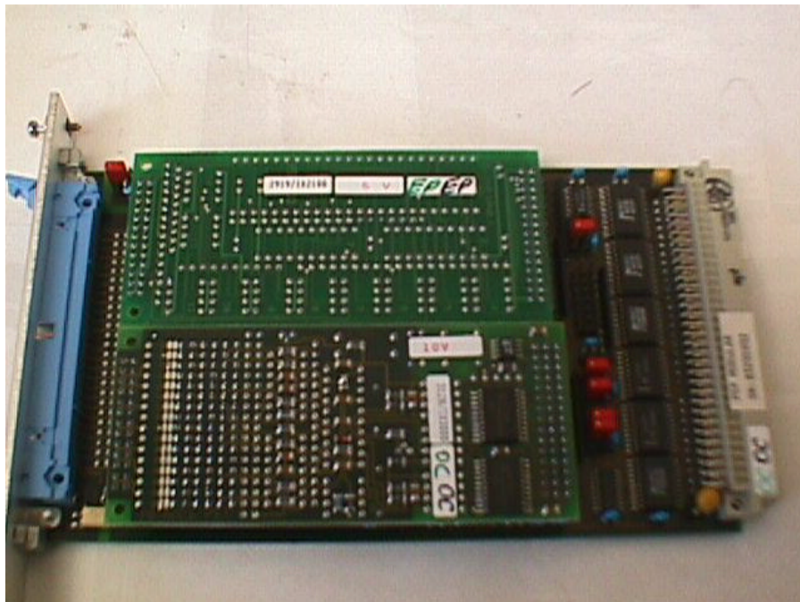
Figure 34: PEP Modular VSBC-4, front
