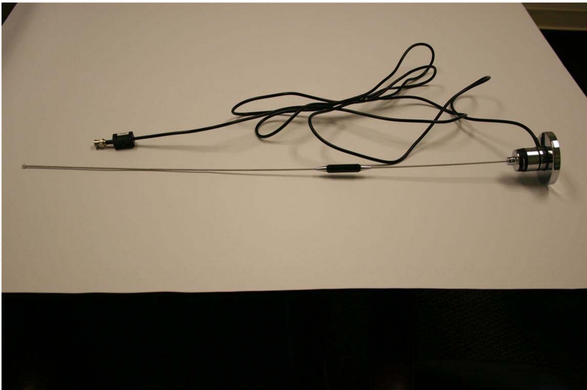
Figure 6: View of the Receive antenna with ferrite at connector end of coax
