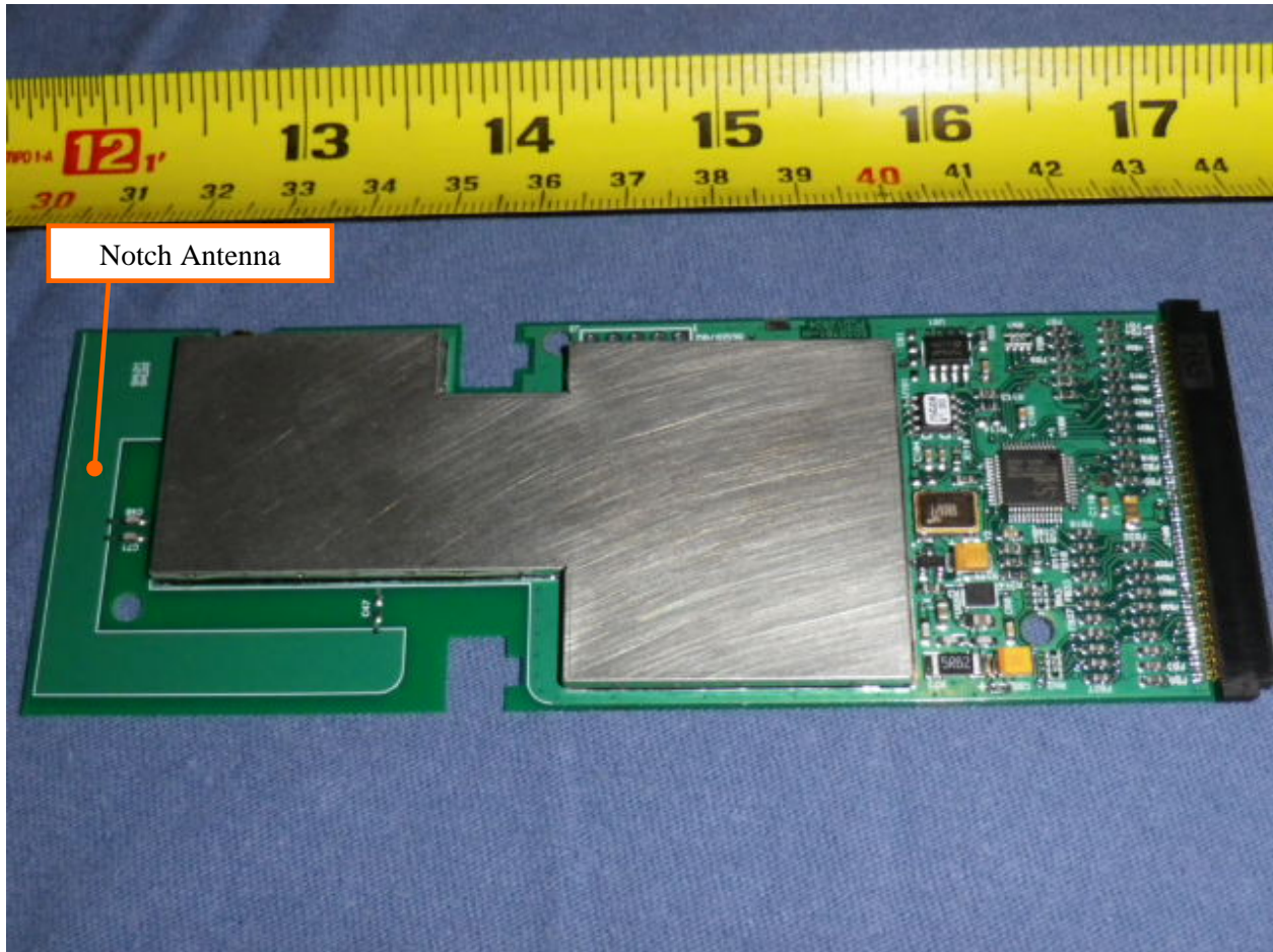
Figure 3: Top view of EUT with shield
