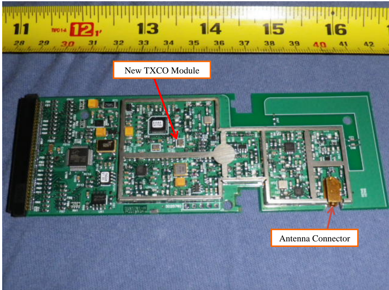
Figure 4: Top view of EUT without shield
