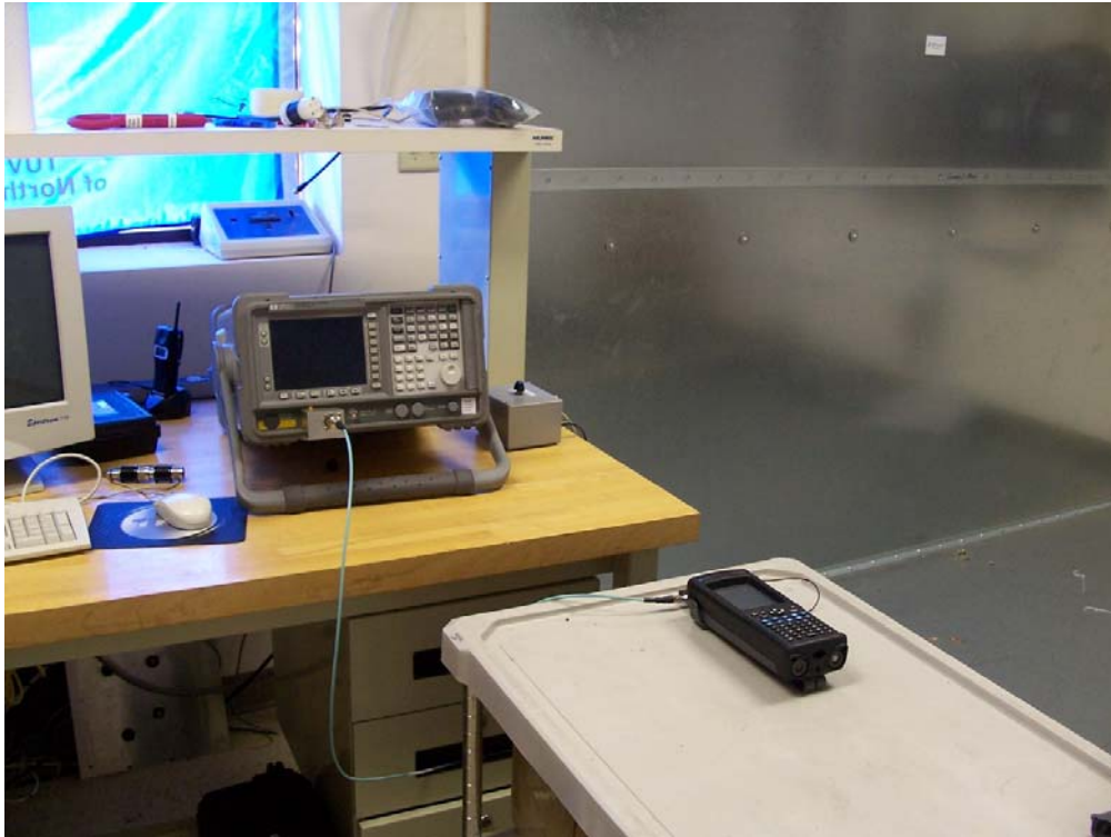
Figure 1: Conducted Power and Emissions Mask Setup
