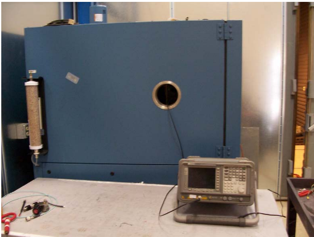
Figure 6: Frequency Stability External Setup
