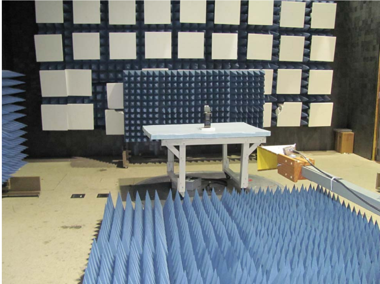
Figure 3: Radiated Emissions at 3m – 1 GHz to 10 GHz.
