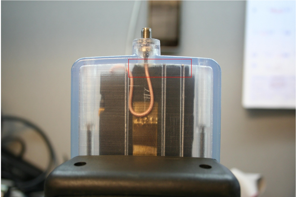
Figure 3: “X-Ray” view of External connector mounting (replacing the PCB antenna)
