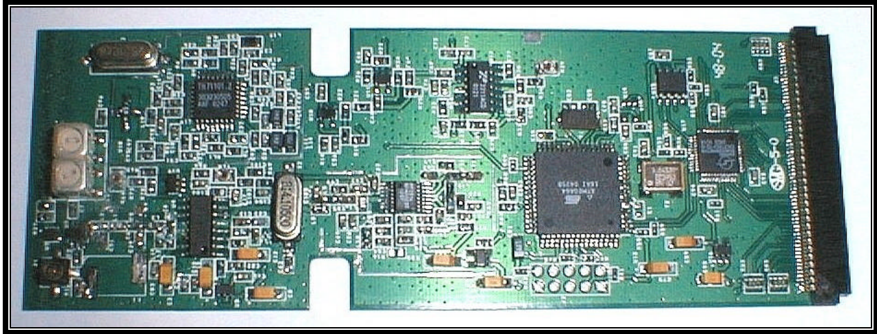
PHOTOGRAPH 4: FRONT WITHOUT SHIELD
