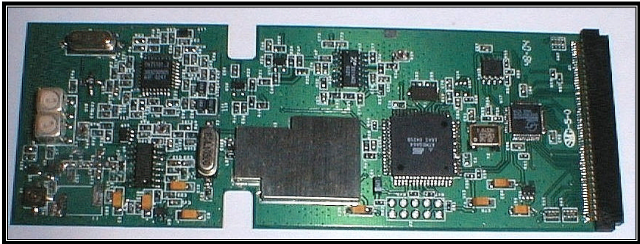
PHOTOGRAPH 5: FRONT WITH SHIELD
