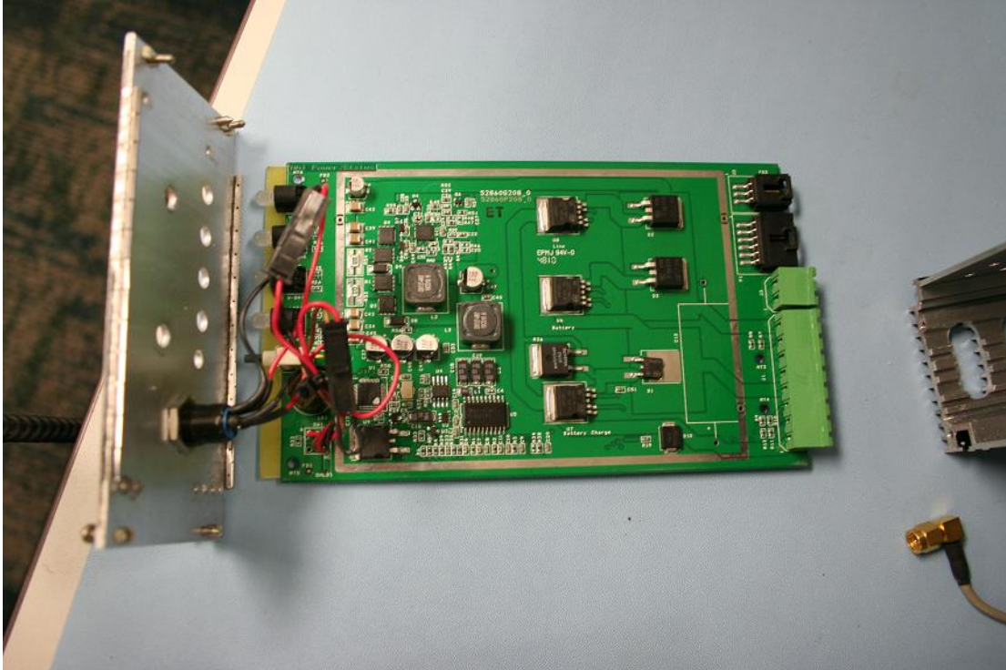
Figure 7: Top view of Power Management Board
