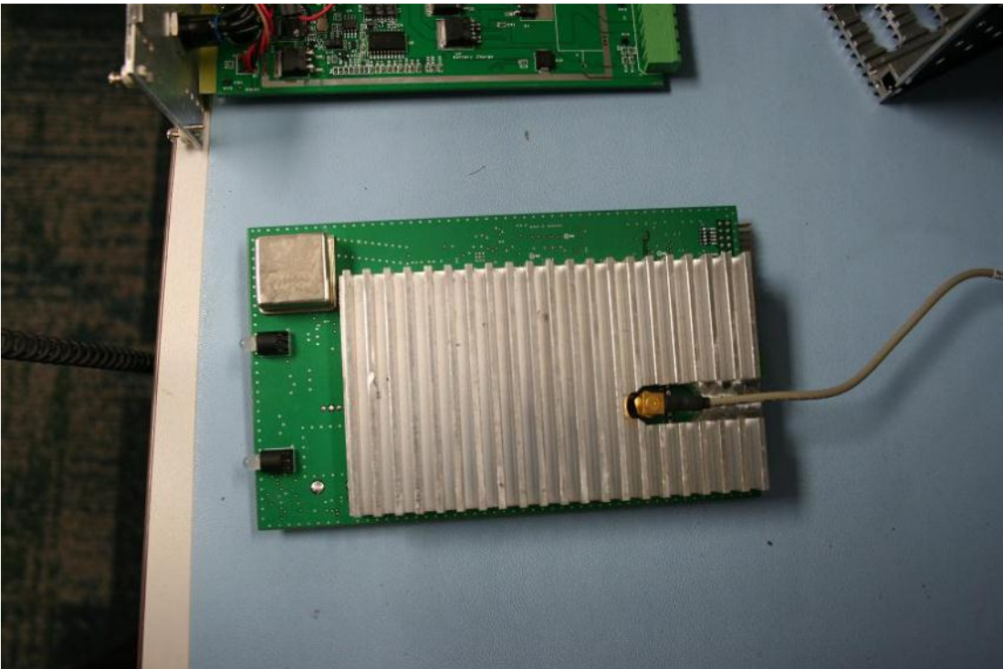
Figure 10: Bottom view of Wake-Up TX board
