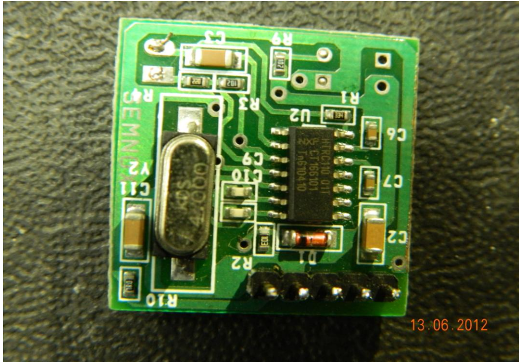
Bottom View of Reader PCB
