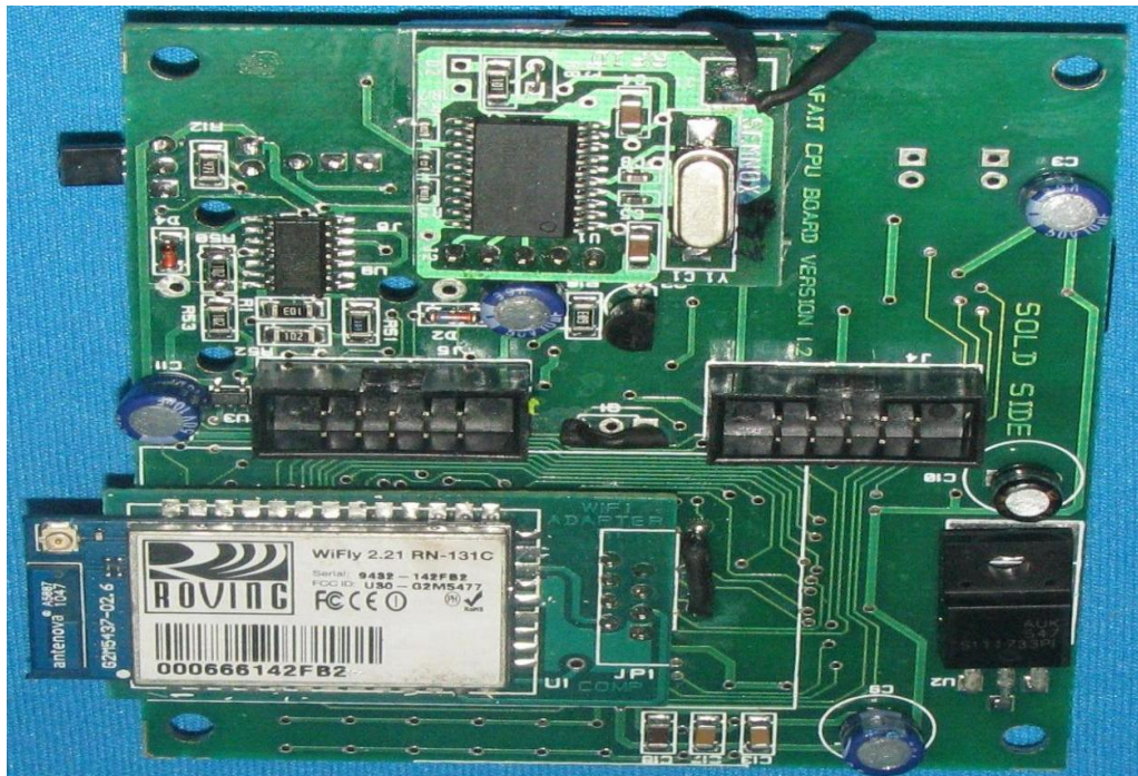
PCB Bottom View Showing Wi-Fi Module
