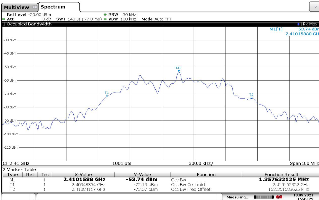
99% OCCUPIED BANDWIDTH LOW CH
