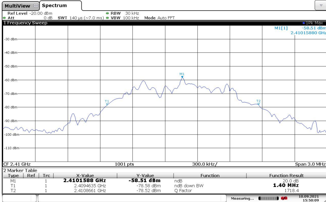
20 dB BANDWIDTH LOW CH
