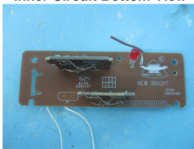
Inner Circuit Bottom View
