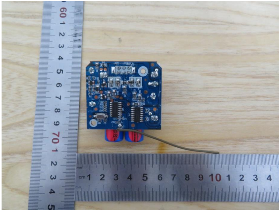
Internal View of EUT-9 (GF64UNRR)
