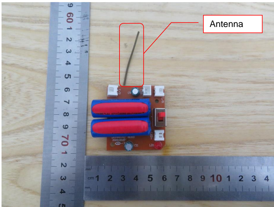
Internal View of EUT-10 (GF64UNRR)
