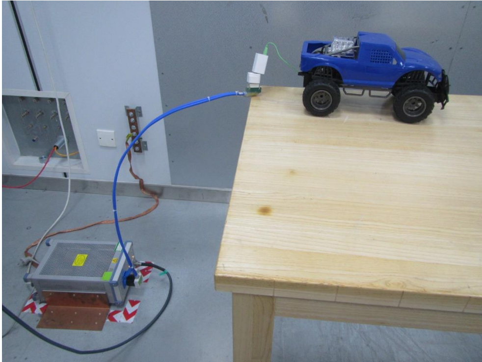
Conducted Disturbance
