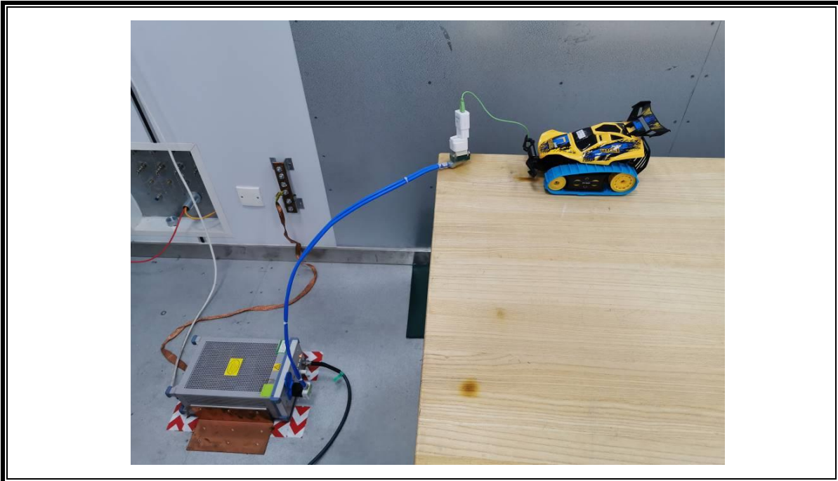
Conducted Emissions test setup photo
